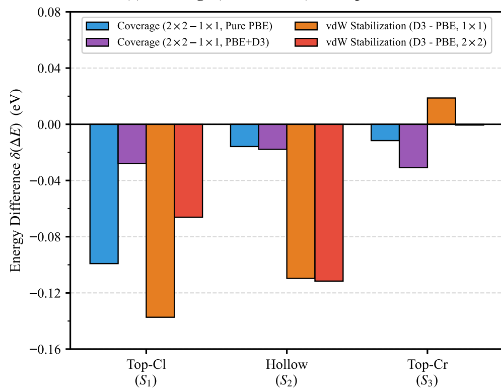
(c) Coverage ( 2 \times 2 vs 1 \times 1 ) & Dispersion Shifts
