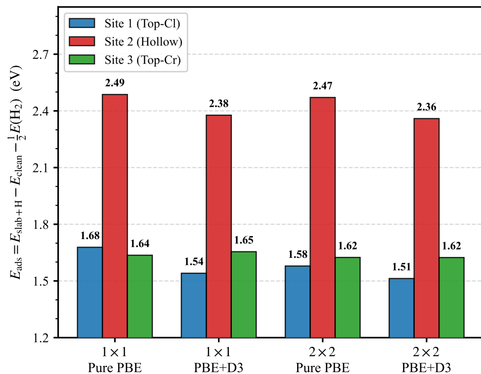
(a) Hydrogen Adsorption Energy vs. Isolated \frac{1}{2}\text{H}_2
