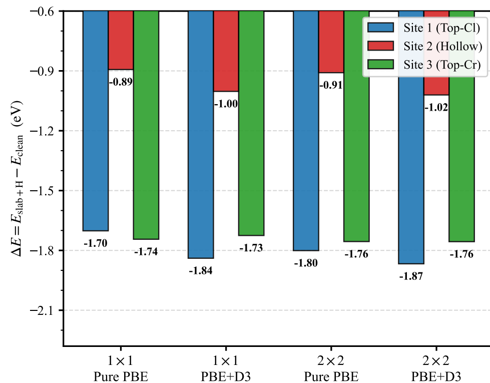
(b) Thermodynamic Binding Energy \Delta E
