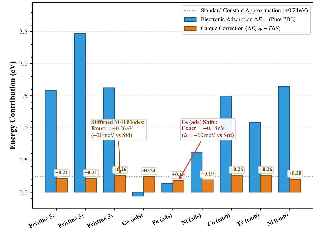
(c) Energy Decomposition: Electronic \Delta E_{\text{ads}} vs. Exact Caique Vibrational Offset
