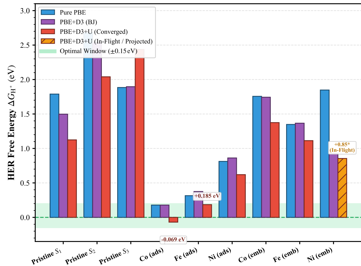
(b) Multilevel Functional Evolution of \Delta G_{\text{H}^*} with Exact Caique Corrections
