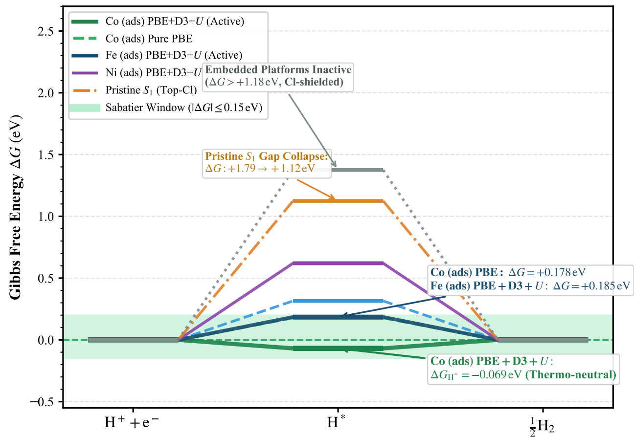
(a) HER Free Energy Reaction Diagram ( T=298.15\text{ K} )
