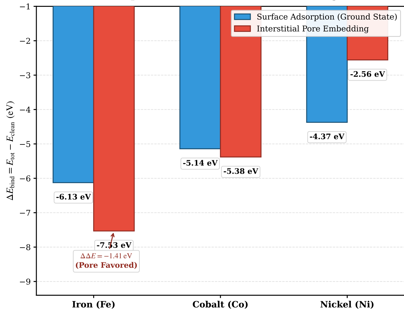
(a) Surface Adsorption vs. Interstitial Pore Embedding ( U_{Cr} = 3.29 eV)
