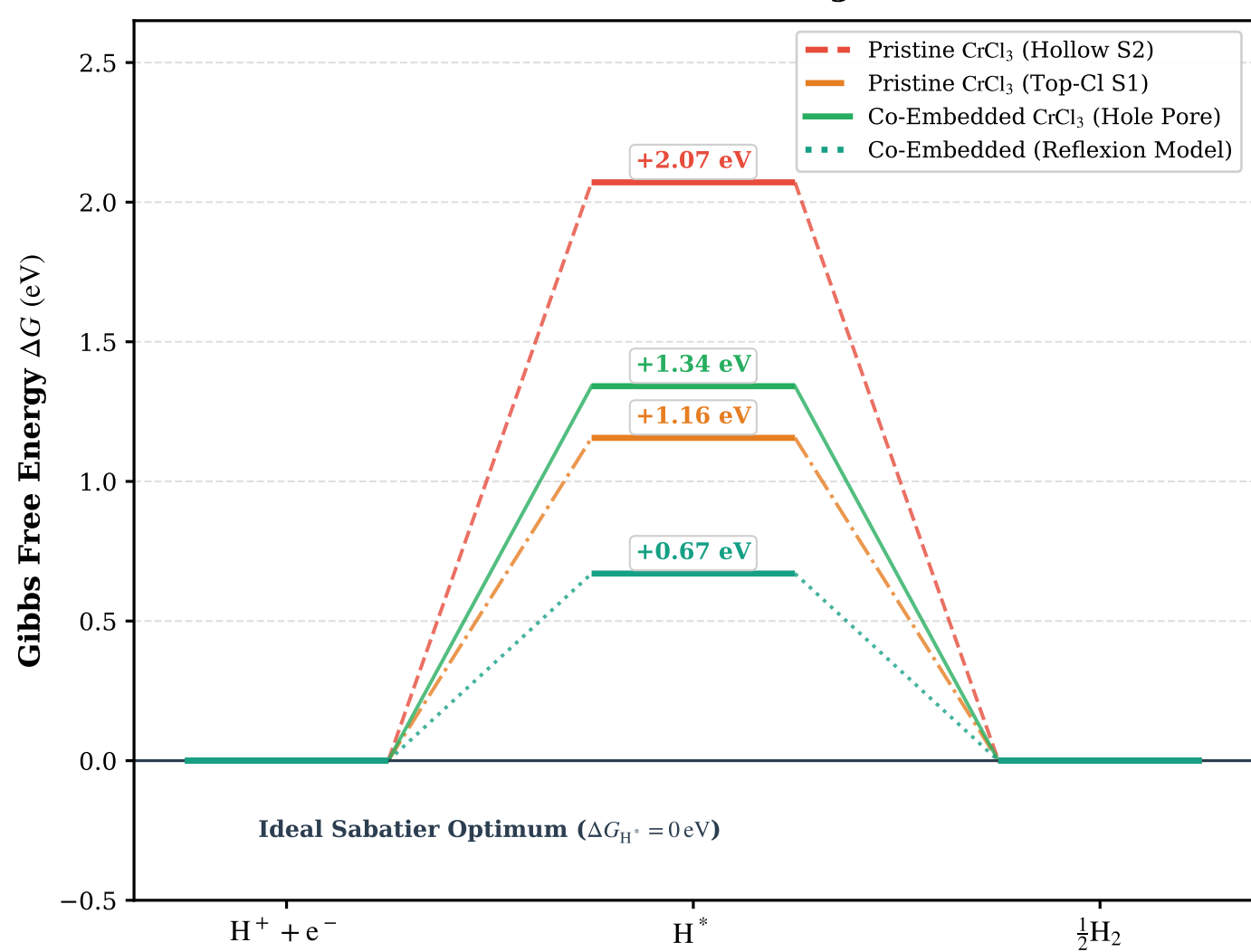
(c) HER Reaction Coordinate Diagram ( T = 298.15 K)
