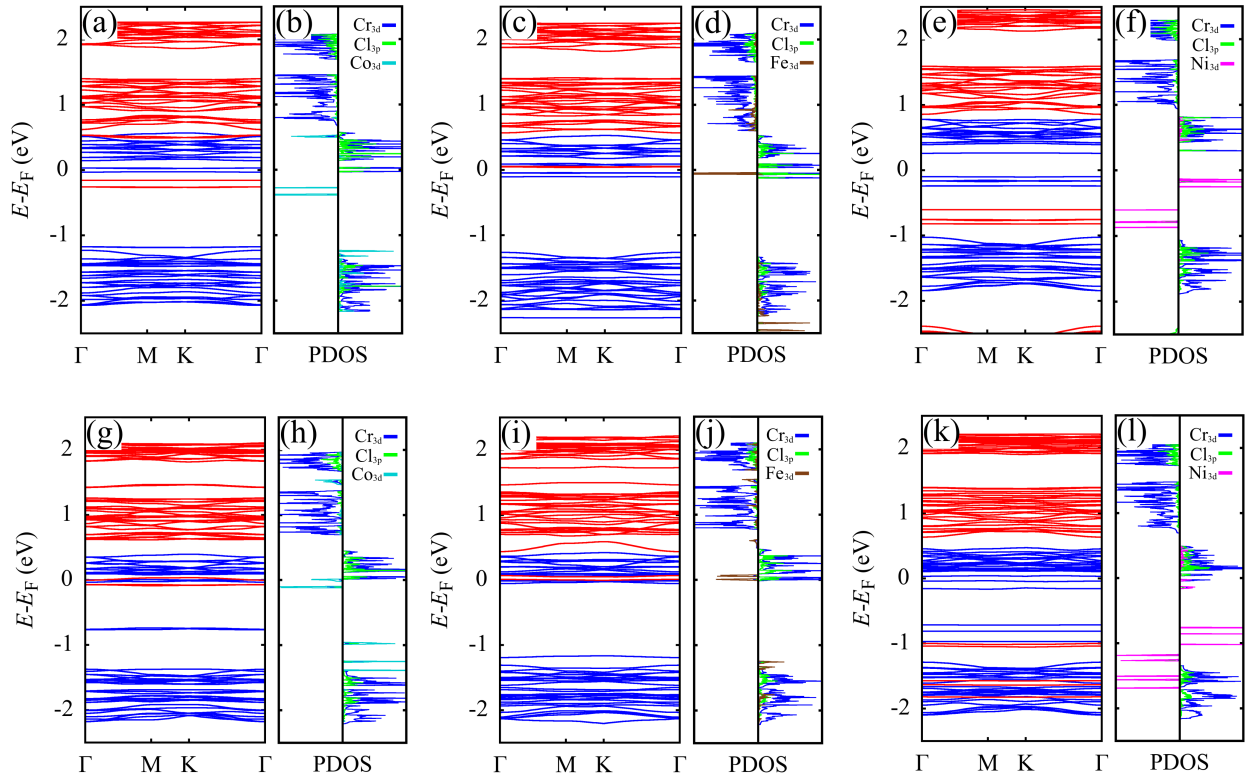
Figure 5: Spin-resolved band structures and projected densities of states of transition-metal-functionalized monolayer CrCl 3 . Panels (a,b), (c,d), and (e,f) correspond to surface-adsorbed Co, Fe, and Ni, respectively; panels (g,h), (i,j), and (k,l) correspond to the embedded configurations. Blue and red bands denote the spin-up and spin-down channels. The PDOS includes Cr-3 d , Cl-3 p , and TM-3 d contributions, and all energies are referenced to the corresponding Fermi level.
