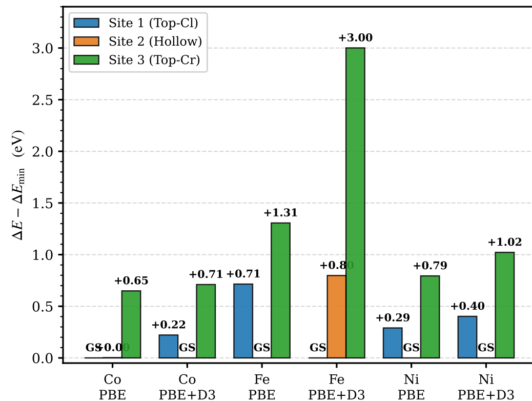
(b) Relative Site Preference & Metastability Penalty
