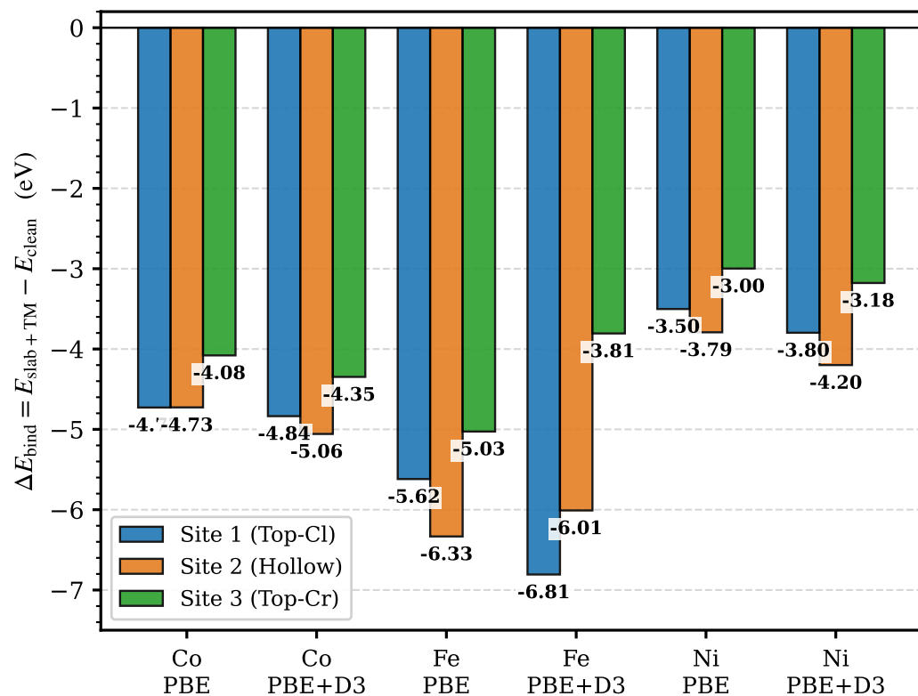
(a) Transition Metal Binding Energy on \text{CrCl}_3 ( 2 \times 2 )
