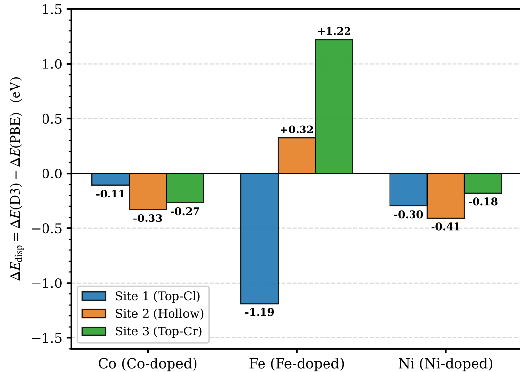
(c) Dispersion Contribution to Binding Energy
