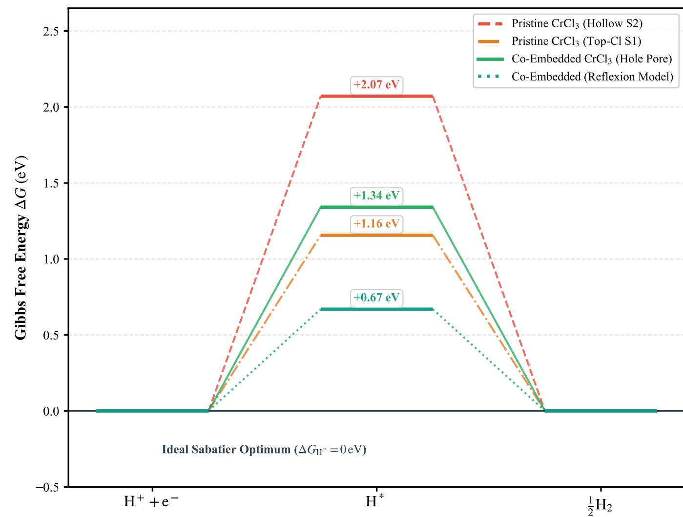
(c) HER Reaction Coordinate Diagram ( T = 298.15 K)
