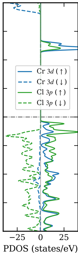
(a) 2 \times 2 \times 1 \text{CrCl}_3 ( +U_{\text{Cr}} , vdW-D3) (b) Projected DOS
