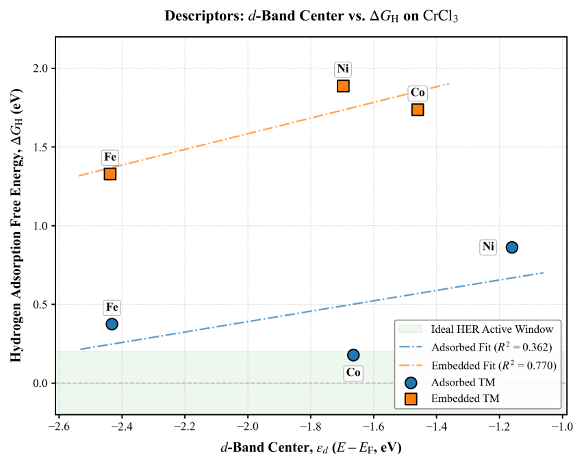
Figure 7: Correlation between the d -band center ( \epsilon_d , E - E_F ) and the hydrogen adsorption free energy ( \Delta G_{\text{H}} ) for adsorbed (blue circles) and embedded (orange squares) transition-metal atoms (Co, Fe, Ni) on \text{CrCl}_3 monolayers. Dashed-dotted lines represent linear regression fits ( R^2 = 0.362 for adsorbed, R^2 = 0.770 for embedded), and the light green shaded band highlights the ideal HER active window ( \Delta G_{\text{H}} \approx 0.0 \pm 0.2 eV).
