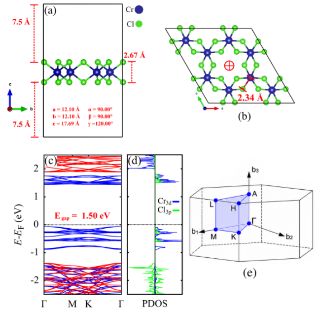
Figure 1: (a) Side view of the optimized pristine \text{CrCl}_3 monolayer, illustrating the atomic configuration and the vacuum spacing ( \sim 15 \text{ \AA} ) introduced along the perpendicular direction to avoid spurious interactions between periodic images. (b) Top view highlighting the Cr-Cl bond lengths and the hollow adsorption site where the transition metals will be incorporated. (c) Electronic band structure of pristine monolayer \text{CrCl}_3 calculated along the high-symmetry path \Gamma -M-K- \Gamma , with the Fermi level aligned at 0 eV. (d) Projected density of states (PDOS), showing the orbital contributions of Cr-3d and Cl-3p states. (e) Schematic representation of the first Brillouin zone of the hexagonal lattice and the selected high-symmetry path used in the electronic-structure calculations.
