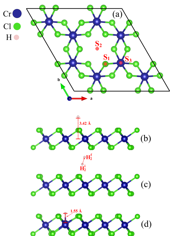
Figure 2: (a) Top view of the pristine CrCl 3 monolayer, showing the three nonequivalent initial adsorption sites considered for a single H atom, labeled as S 1 , S 2 , and S 3 . (b-d) Side views of the relaxed adsorption geometries obtained after placing H at the S 1 , S 2 , and S 3 sites, respectively. These panels illustrate the distinct adsorption behaviors after structural relaxation and the corresponding equilibrium distances between the H atom and the CrCl 3 monolayer.
