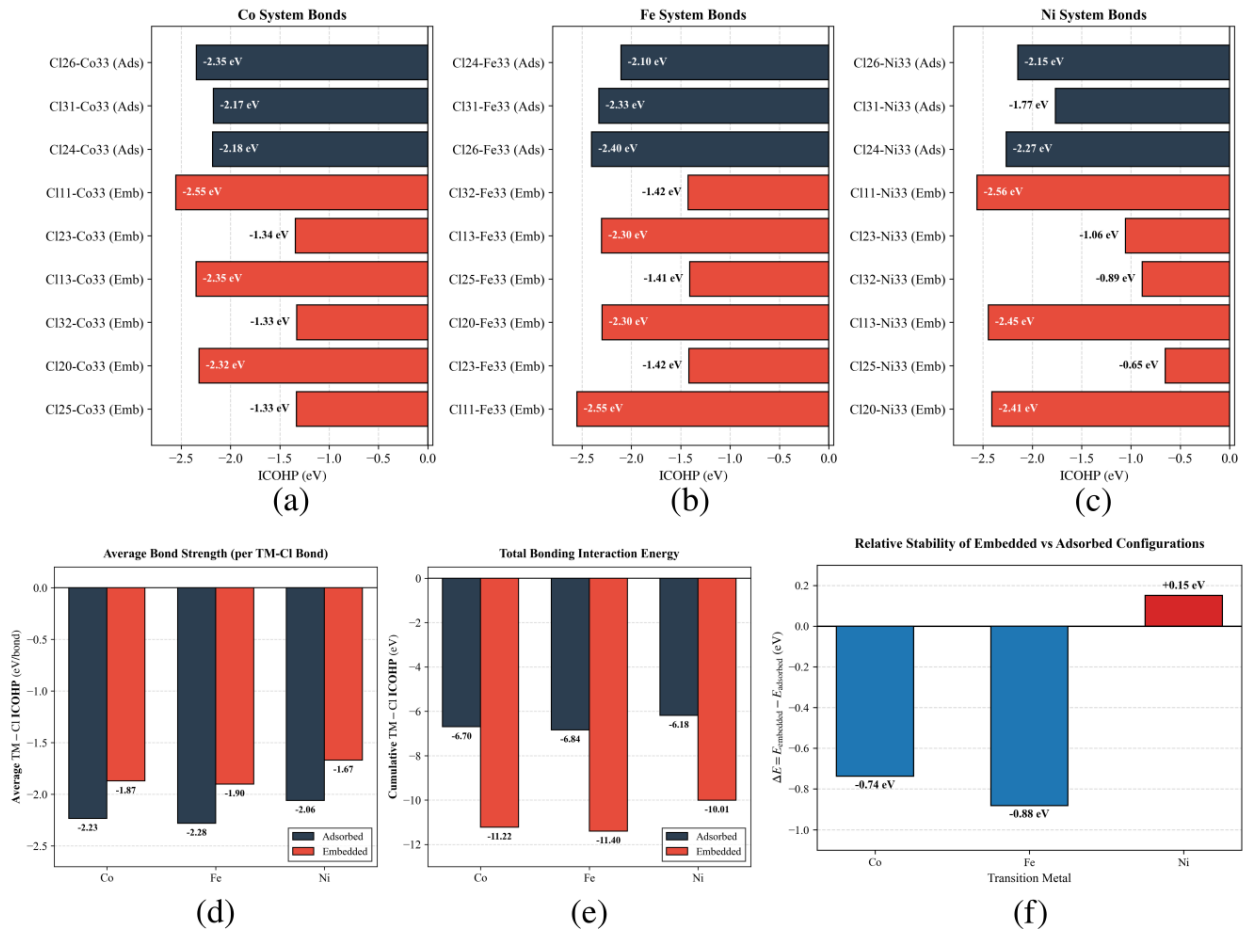
Figure 6: LOBSTER Integrated Crystal Orbital Hamilton Population (ICOHP) chemical bonding analysis and relative stability of embedded versus adsorbed configurations for Co-, Fe-, and Ni-functionalized \text{CrCl}_3 monolayers. (a–c) Individual TM–Cl ICOHP bond energy values (eV) for 3-fold coordinated adsorbed and 6-fold octahedrally coordinated embedded Co, Fe, and Ni systems, respectively. (d) Average bond strength per TM–Cl bond. (e) Total cumulative bonding interaction energy summed over all TM–Cl bonds. (f) Relative energy stability ( \Delta E = E_{\text{embedded}} - E_{\text{adsorbed}} ) for embedded versus adsorbed transition-metal configurations.
