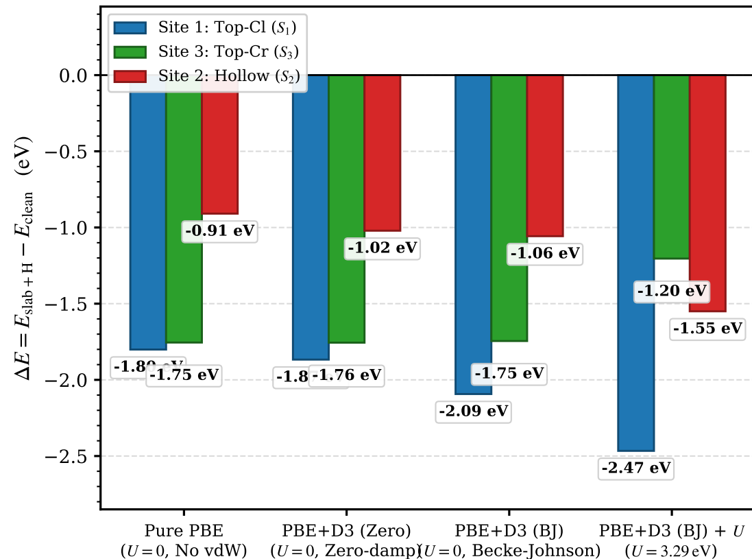
(b) Thermodynamic Binding Energy ( \Delta E )
