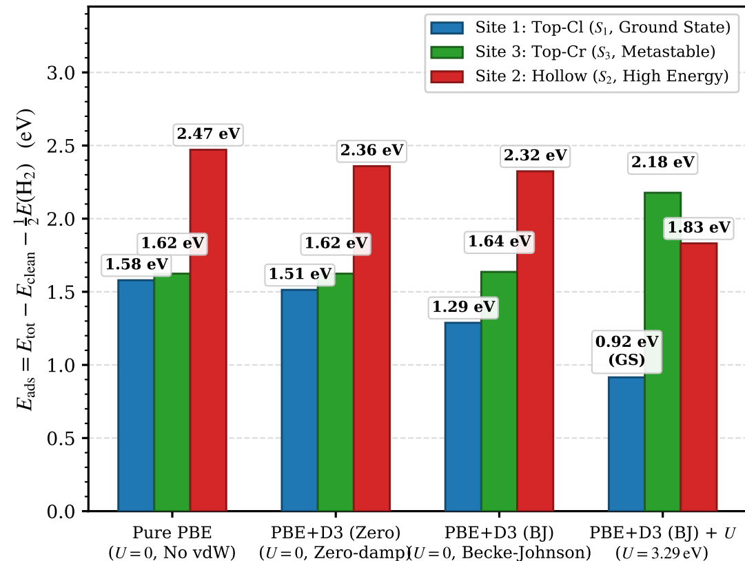
(a) 2 \times 2 Hydrogen Adsorption Energy ( E_{\text{ads}} )
