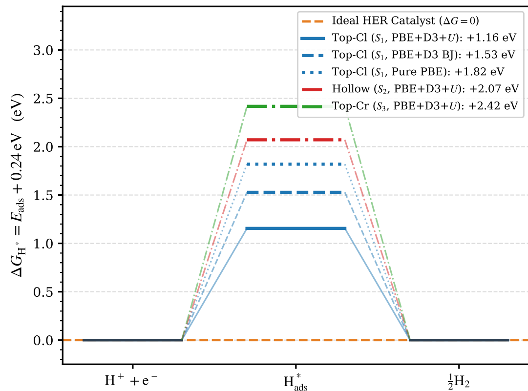
(c) 2 \times 2 HER Free Energy Profile ( \theta = 0.25 )
