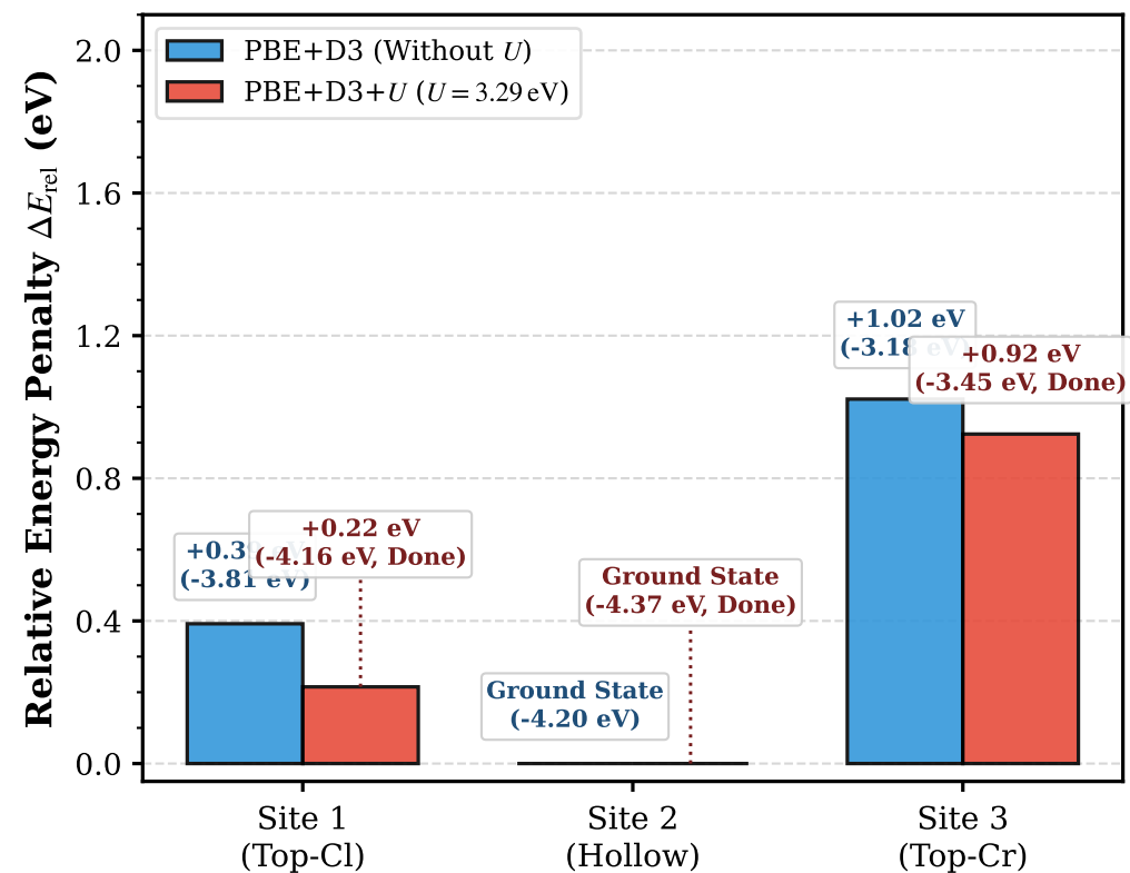
(a) Ni Adsorption Site Preference on \text{CrCl}_3(2 \times 2)
