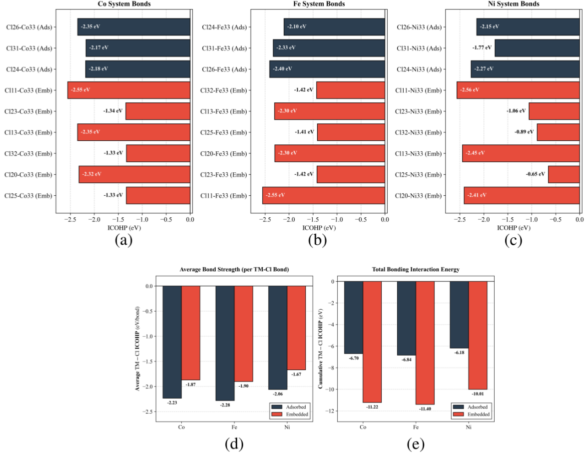
Fig. S4. TM-Cl chemical-bonding analysis and relative stability of surface-adsorbed and embedded transition-metal configurations in monolayer \text{CrCl}_3 . (a-c) Individual integrated crystal orbital Hamilton population (ICOHP) values for the Co-Cl, Fe-Cl, and Ni-Cl interactions, respectively. Dark bars correspond to the threefold coordinated surface-adsorbed configurations, whereas red bars correspond to the sixfold coordinated embedded configurations. More negative ICOHP values indicate stronger net bonding interactions. (d) Average ICOHP per TM-Cl bond for the adsorbed and embedded configurations. (e) Cumulative TM-Cl ICOHP obtained by summing the individual ICOHP contributions over the corresponding coordination shell.
