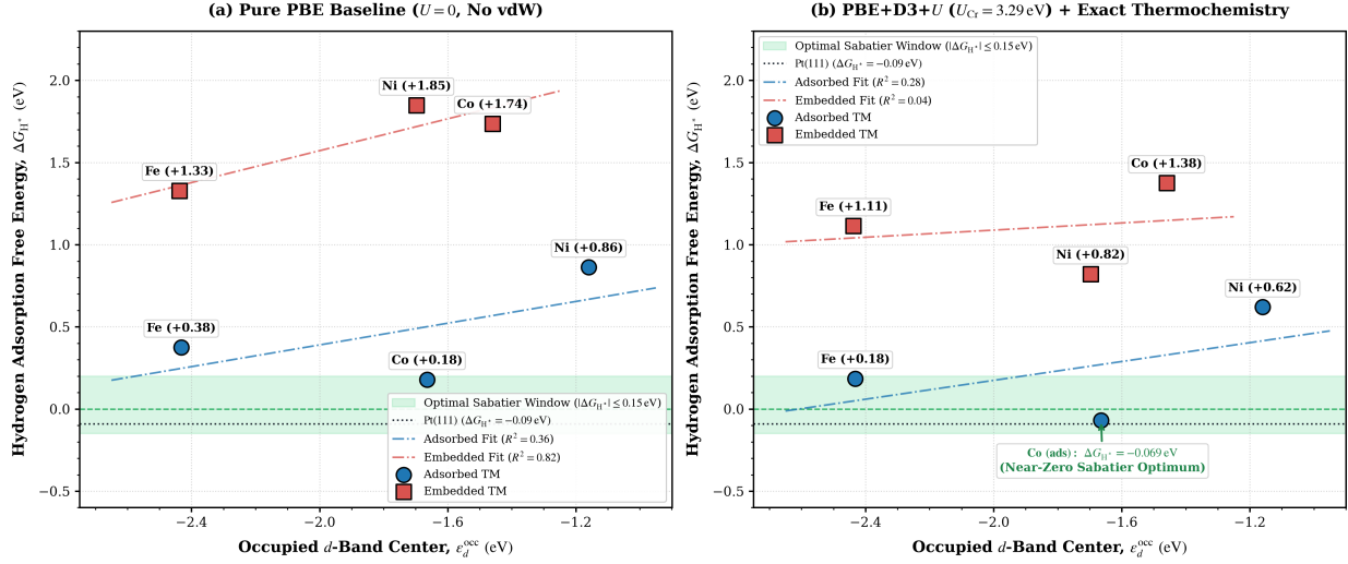
Figure 8: Occupied d -band center, \epsilon_d^{\text{occ}} , versus hydrogen adsorption free energy, \Delta G_{\text{H}^*} , for surface-adsorbed and embedded Co, Fe, and Ni centers in monolayer \text{CrCl}_3 under (a) pure PBE baseline and (b) PBE+D3+U ( U_{\text{Cr}} = 3.29 eV) with explicit vibrational zero-point and entropic corrections. Linear fits are included only as visual guides because each coordination family contains three data points. Shaded green bands denote the optimal Sabatier catalytic window ( |\Delta G_{\text{H}^*}| \leq 0.15 eV) with the Pt(111) benchmark ( -0.09 eV) indicated by dotted horizontal lines.
