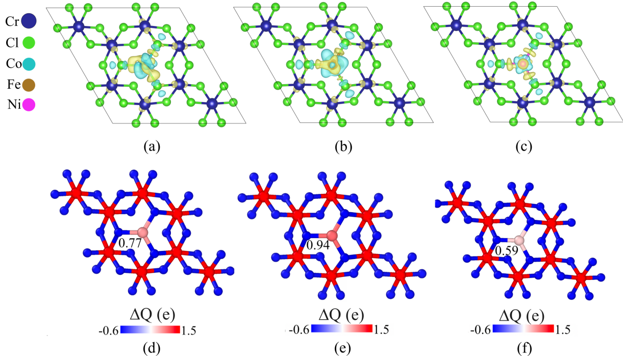
Figure 4: Charge redistribution induced by transition-metal adsorption on monolayer CrCl 3 . (a–c) Charge-density-difference isosurfaces for surface-adsorbed Co, Fe, and Ni, plotted at \delta = 5 \times 10^{-3} e/\text{\AA}^3 . (d–f) Corresponding Bader charge-variation maps. Blue and red regions denote electron depletion and accumulation, respectively; the numerical labels indicate the charge-transfer magnitude associated with each transition-metal atom.
