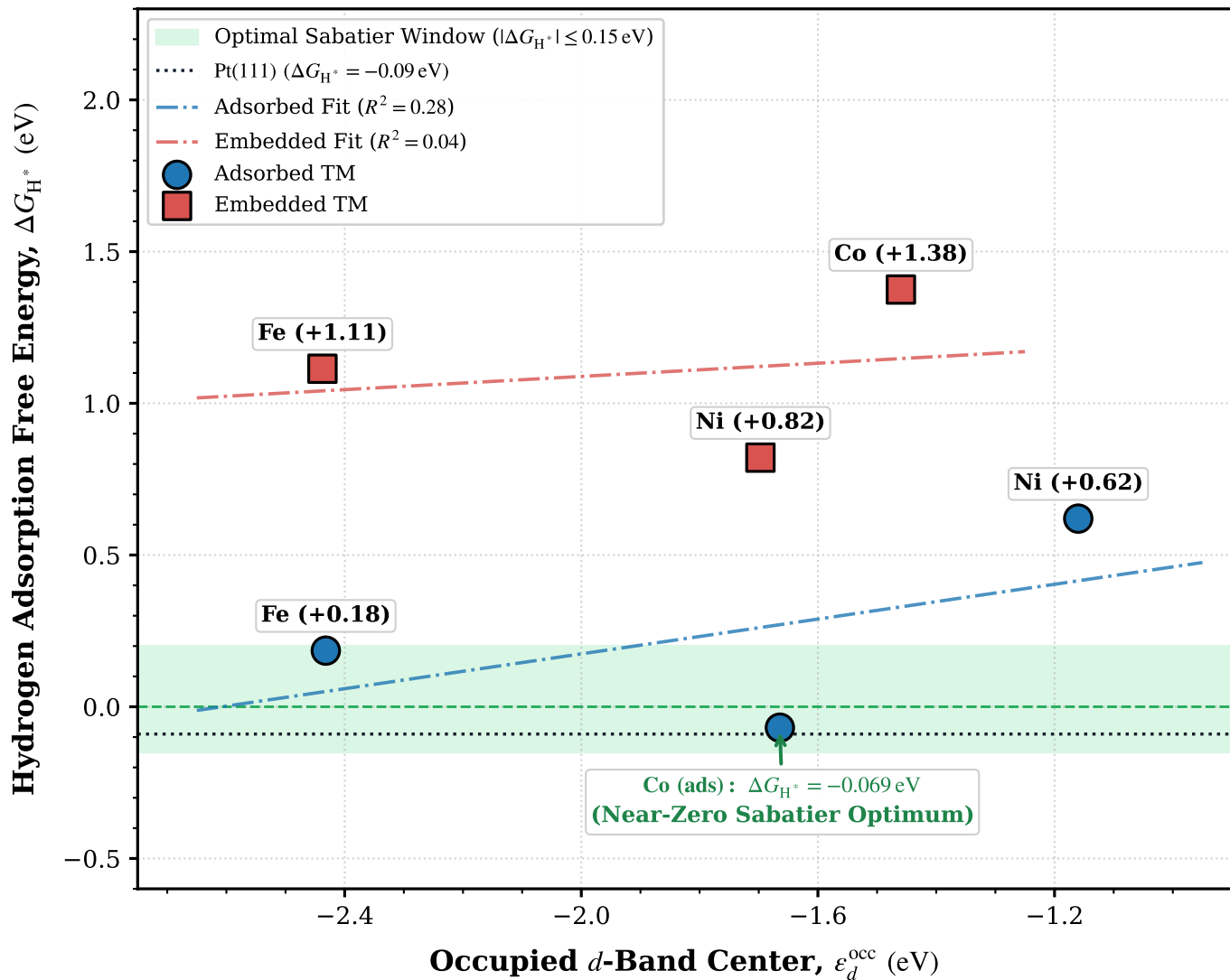
(b) PBE+D3+ U ( U_{\text{Cr}} = 3.29 eV) + Exact Thermochemistry
