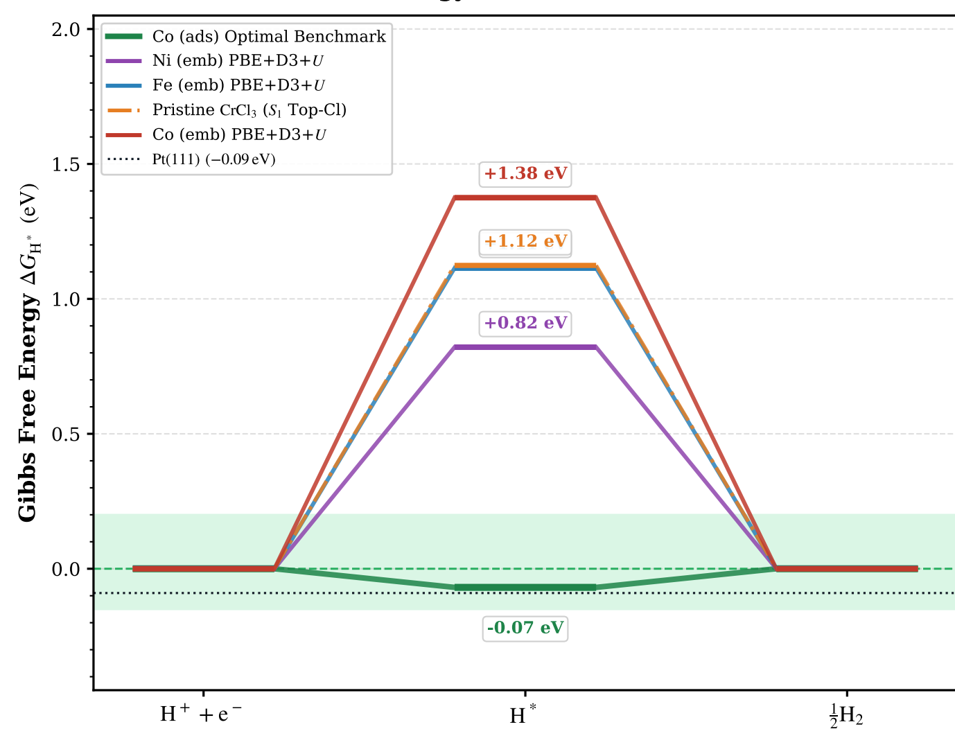
(c) HER Free Energy Reaction Profiles ( T = 298.15 K)
