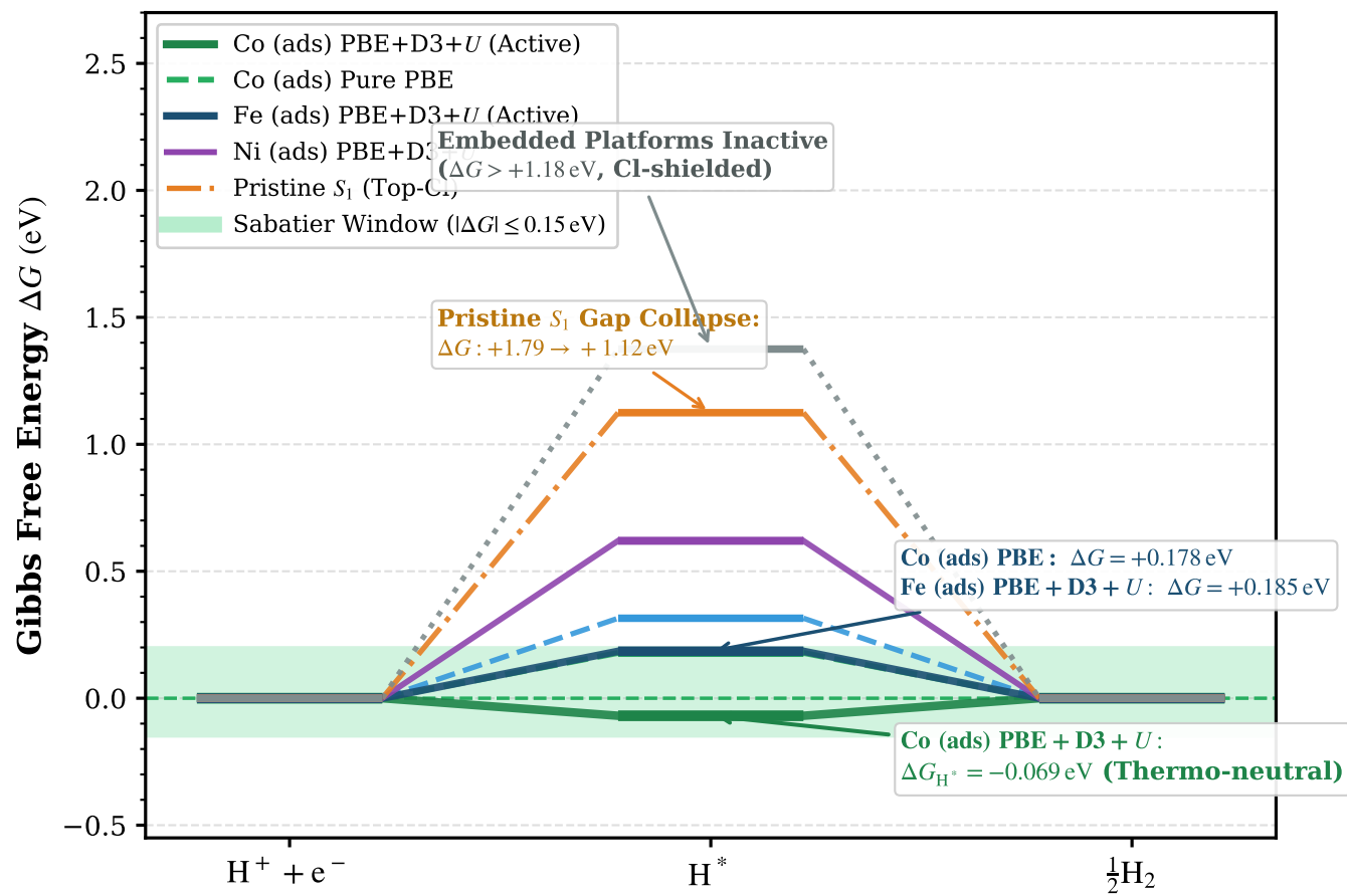
(a) HER Free Energy Reaction Diagram ( T=298.15\text{ K} )
