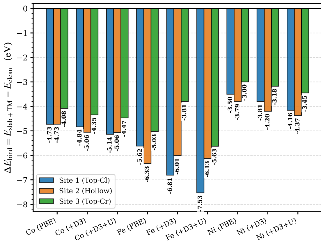
(a) Transition Metal Binding Energy on CrCl 3 (2 × 2)
