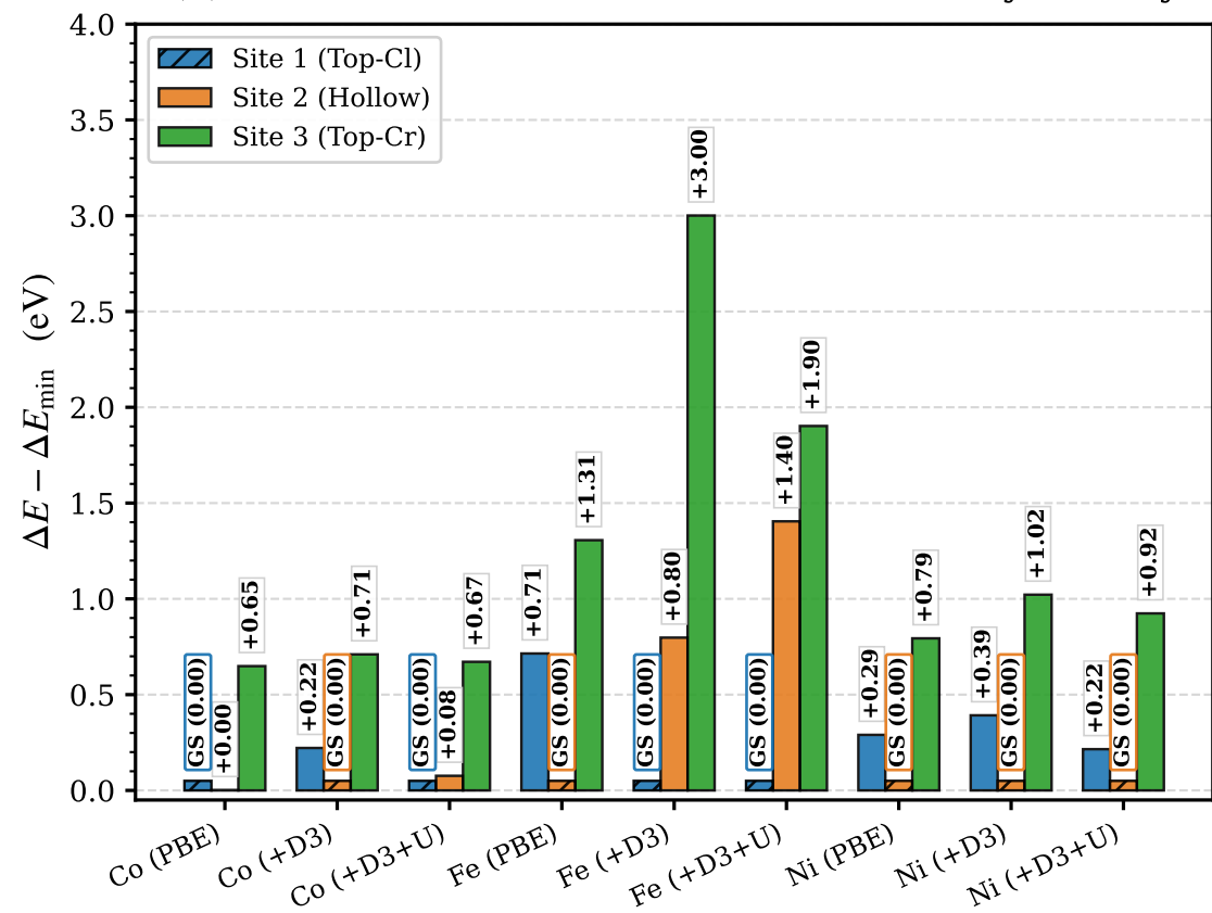
(b) Relative Site Preference & Metastability Penalty
