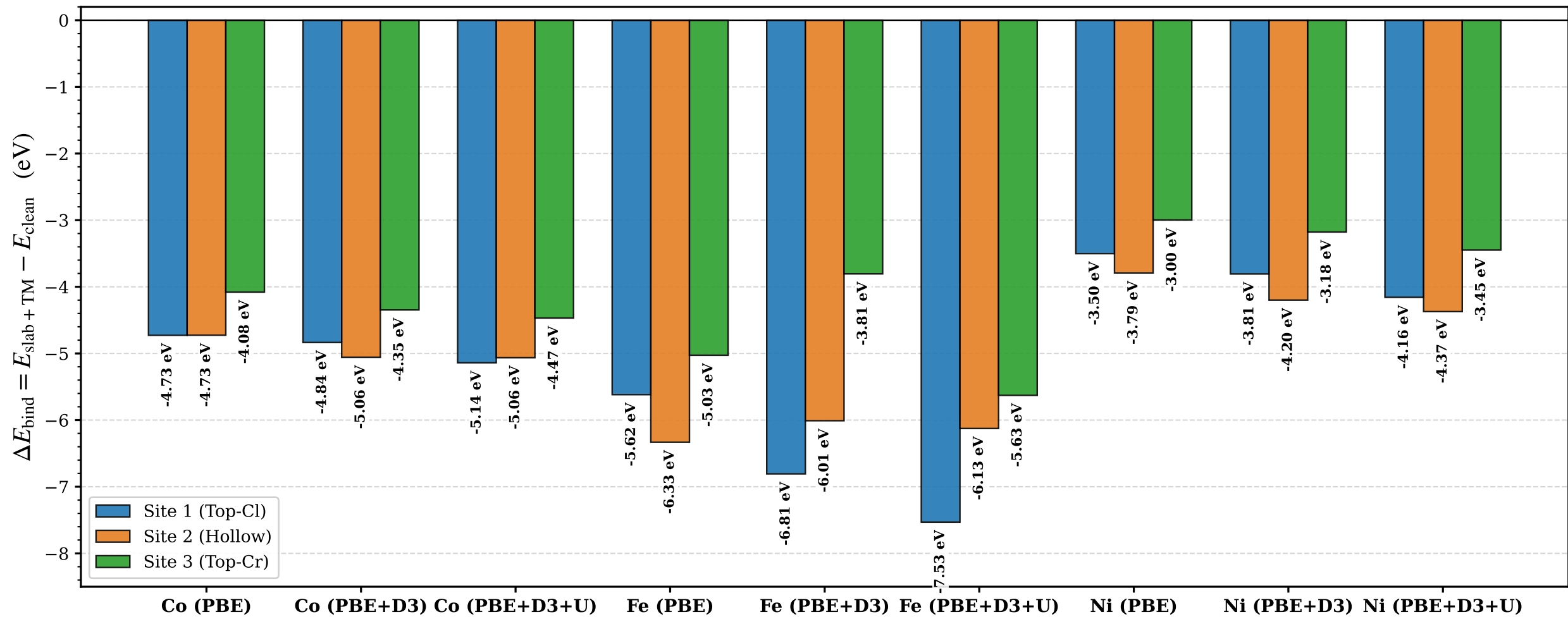
Adsorption Energetics and Site Competition for 3d Transition Metals on Monolayer CrCl 3
