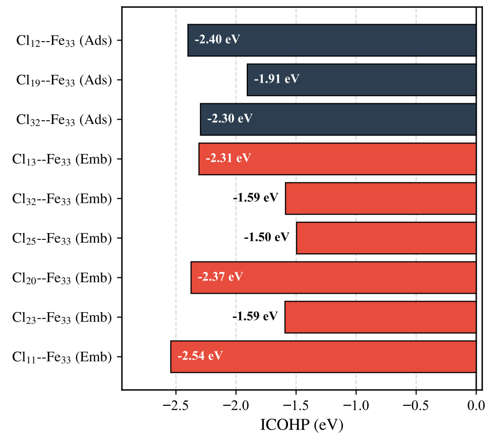
Fe System Bonds
