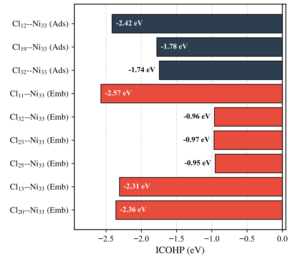
Ni System Bonds
