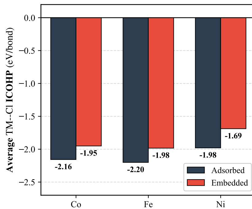
Average Bond Strength (per TM--Cl Bond)
