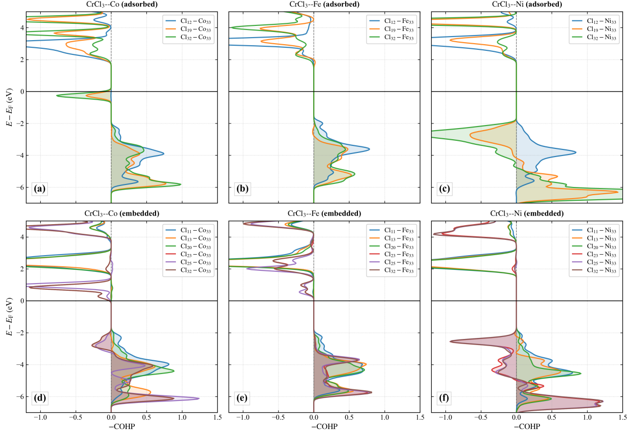
Figure 6: Energy-resolved -\text{COHP} curves for individual TM-Cl bonds in transition-metal-functionalized monolayer \text{CrCl}_3 under multi-site +U_{\text{all}} ( U_{\text{Cr}} = U_{\text{TM}} = 3.29 eV). (a-c) Surface-adsorbed Co, Fe, and Ni in threefold coordination at the S_2 hollow site. (d-f) Embedded Co, Fe, and Ni in distorted sixfold coordination. The horizontal line marks the Fermi level. Positive -\text{COHP} values denote bonding contributions and negative values denote antibonding contributions.
