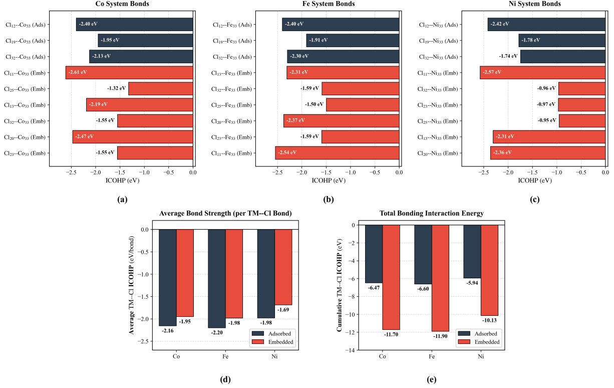
Fig. S4. TM-Cl chemical-bonding analysis and relative stability of surface-adsorbed and embedded transition-metal configurations in monolayer CrCl 3 under the multi-site +U_{\text{all}} tier ( U_{\text{Cr}} = U_{\text{TM}} = 3.29 eV; consistent with Figure 6, with full Pure PBE and +U_{\text{all}} comparisons consolidated in Table S4). (a-c) Individual integrated crystal orbital Hamilton population (ICOHP) values for the Co-Cl, Fe-Cl, and Ni-Cl interactions, respectively. Dark navy bars correspond to the threefold coordinated surface-adsorbed configurations at the S_2 hollow site, whereas red bars correspond to the sixfold coordinated embedded configurations. More negative ICOHP values indicate stronger net bonding interactions. (d) Average ICOHP per TM-Cl bond for the adsorbed and embedded configurations. (e) Cumulative TM-Cl ICOHP obtained by summing the individual ICOHP contributions over the corresponding coordination shell.
