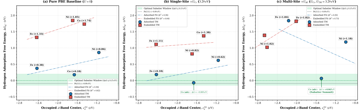
Figure 8: Occupied d -band center, \varepsilon_d^{\text{occ}} , versus hydrogen adsorption free energy, \Delta G_{\text{H}^*} , for surface-adsorbed and embedded Co, Fe, and Ni centers in monolayer \text{CrCl}_3 under (a) pure PBE baseline and (b) PBE+D3+ U ( U_{\text{Cr}} = 3.29 eV; with + U_{\text{all}} benchmark in Table 1) with explicit vibrational zero-point and entropic corrections. Linear fits are included only as visual guides because each coordination family contains three data points. Shaded green bands denote the optimal Sabatier catalytic window ( |\Delta G_{\text{H}^*}| \leq 0.15 eV) with the Pt(111) benchmark ( -0.09 eV) indicated by dotted horizontal lines.
