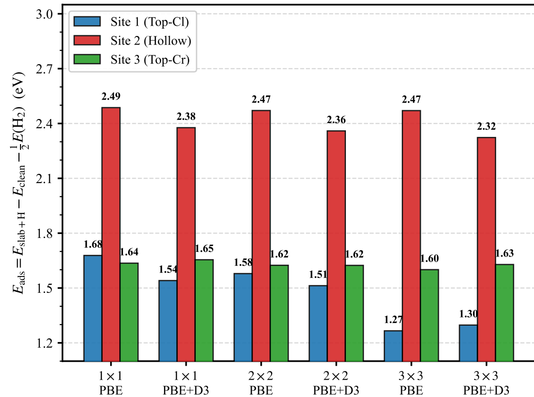
(a) Hydrogen Adsorption Energy ( 1 \times 1 vs 2 \times 2 vs 3 \times 3 )
