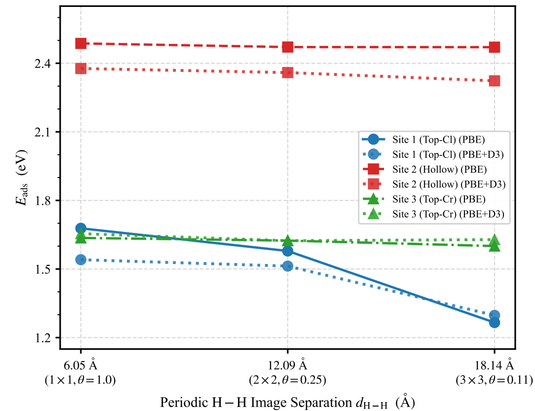
(c) Multi-Scale Coverage Convergence: E_{\text{ads}} vs d_{\text{H-H}}
