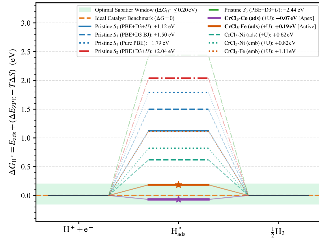
(c) 2 \times 2 HER Free Energy Profile: Pristine vs TM Activation
