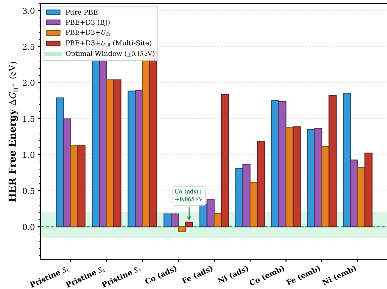
(b) 4-Tier Evolution of \Delta G_{\text{H}^*} with Exact Caique Corrections
