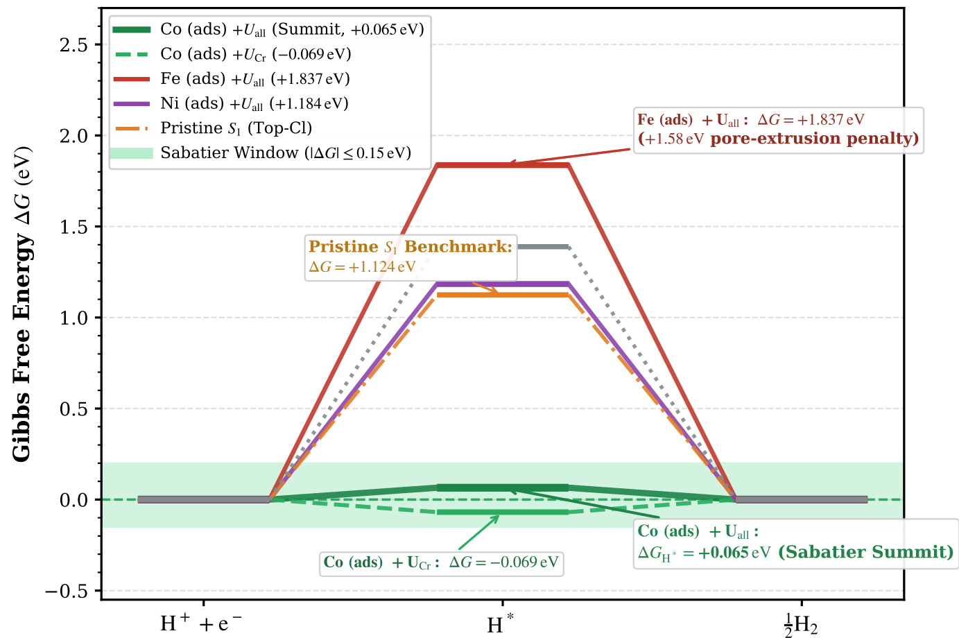
(a) HER Free Energy Reaction Diagram ( T = 298.15 K)
