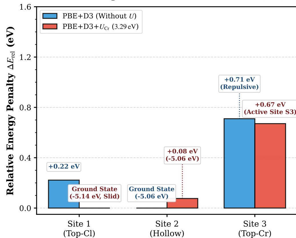
(a) Co Adsorption Site Preference on \text{CrCl}_3(2 \times 2)
