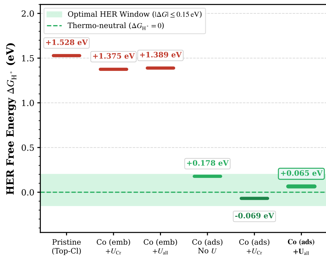
(c) Co HER Descriptor Benchmarks (+ U_{\text{Cr}} vs + U_{\text{all}} )
