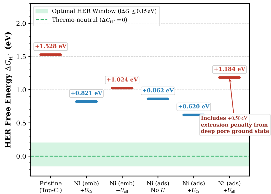
(c) Ni HER Electrocatalytic Descriptor Benchmarks
