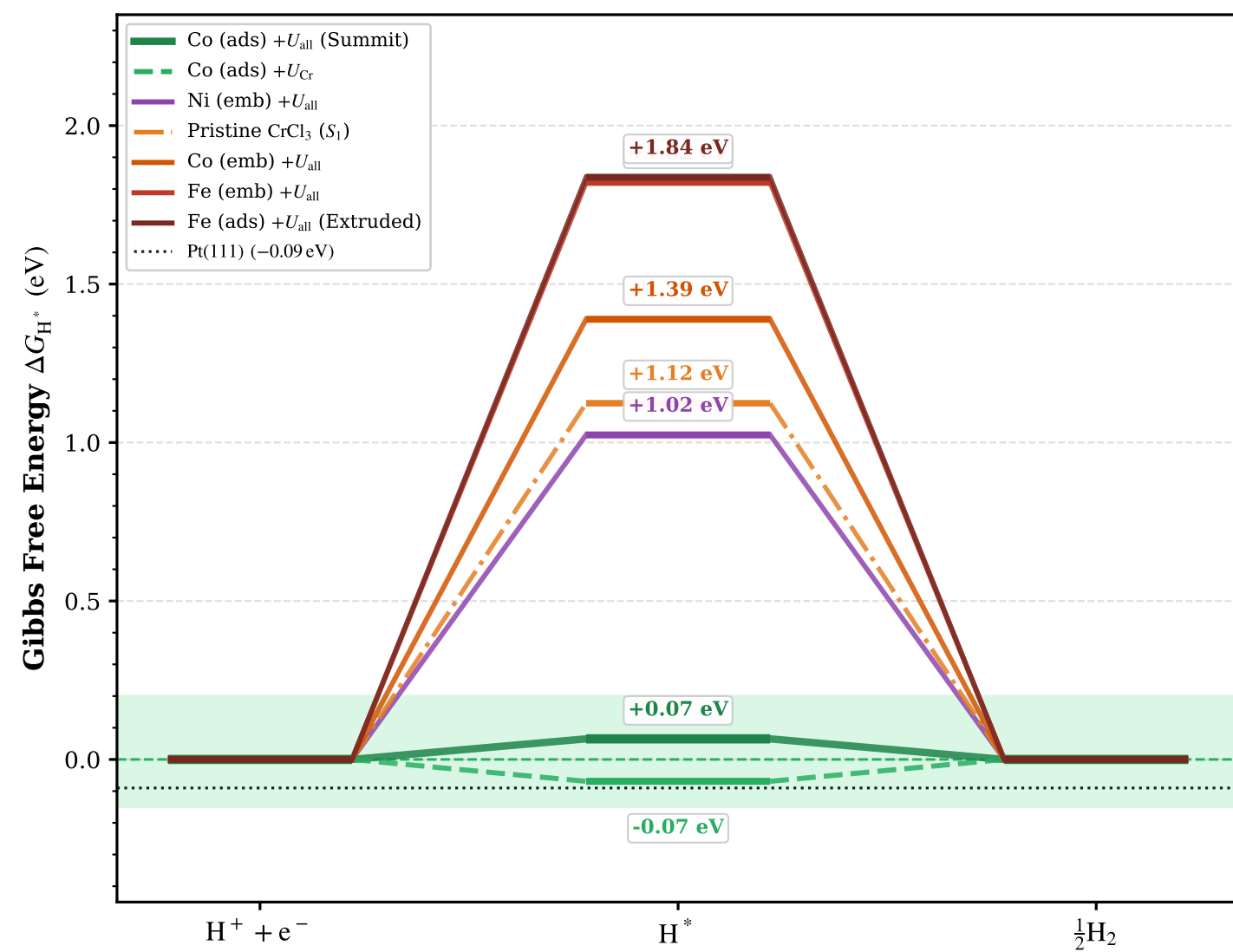
(c) HER Free Energy Reaction Profiles across Tiers
