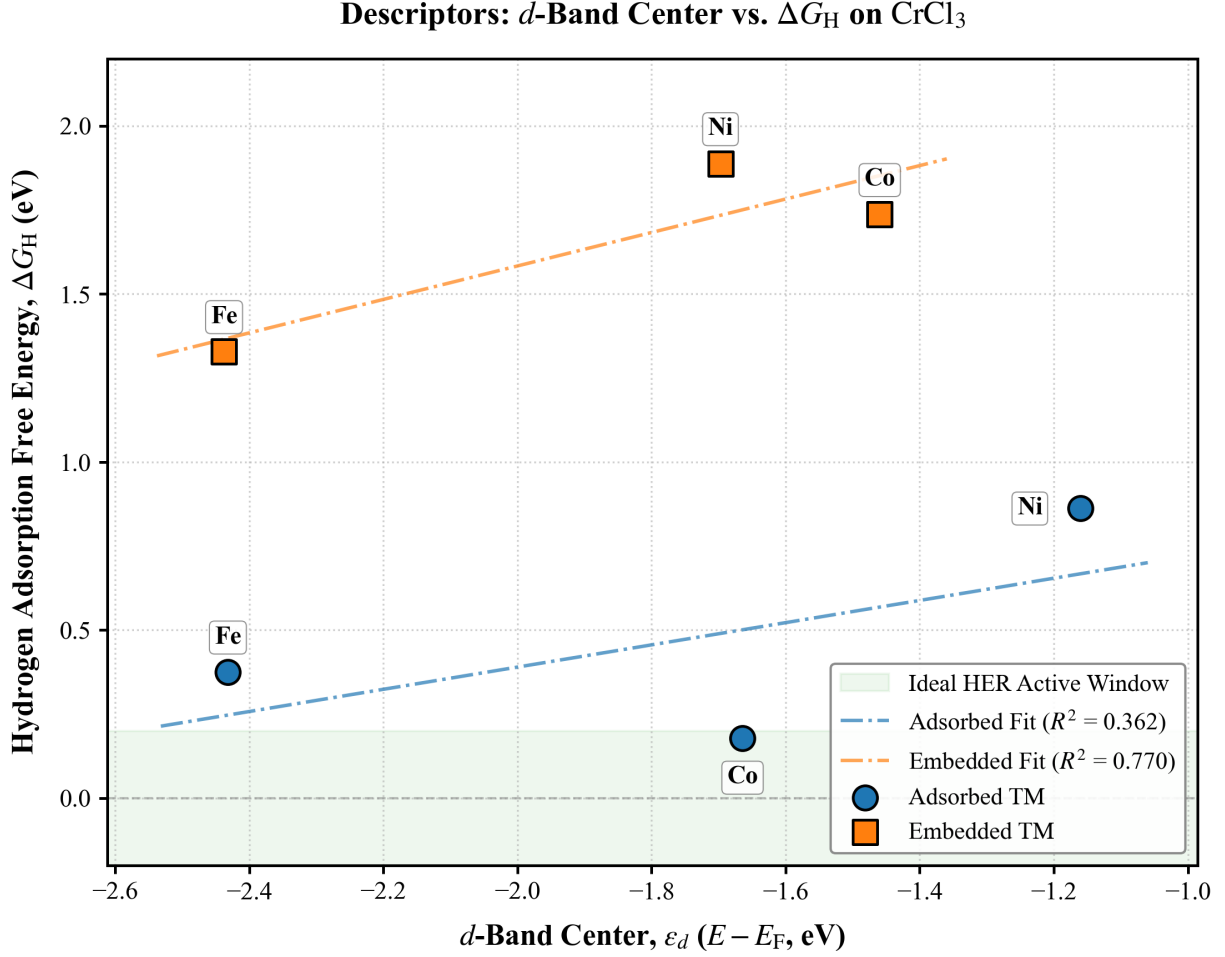
Figure 8: Occupied d -band center, \epsilon_d^{\text{occ}} , versus H adsorption free energy, \Delta G_{\text{ads}} , for surface-adsorbed and embedded Co, Fe, and Ni centers in monolayer \text{CrCl}_3 . The linear fits are included only as visual guides because each coordination family contains three data points. The shaded region denotes -0.2 \leq \Delta G_{\text{ads}} \leq 0.2 eV.
