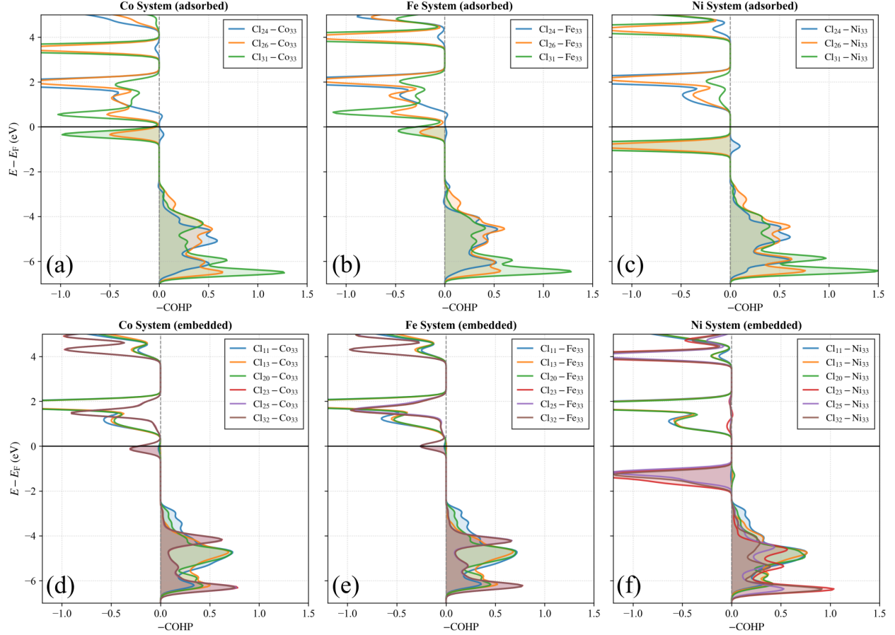
Figure 6: Energy-resolved -\text{COHP} curves for individual TM-Cl bonds in transition-metal-functionalized monolayer \text{CrCl}_3 . (a-c) Surface-adsorbed Co, Fe, and Ni in threefold coordination. (d-f) Embedded Co, Fe, and Ni in distorted sixfold coordination. The horizontal line marks the Fermi level. Positive -\text{COHP} values denote bonding contributions and negative values denote antibonding contributions.
