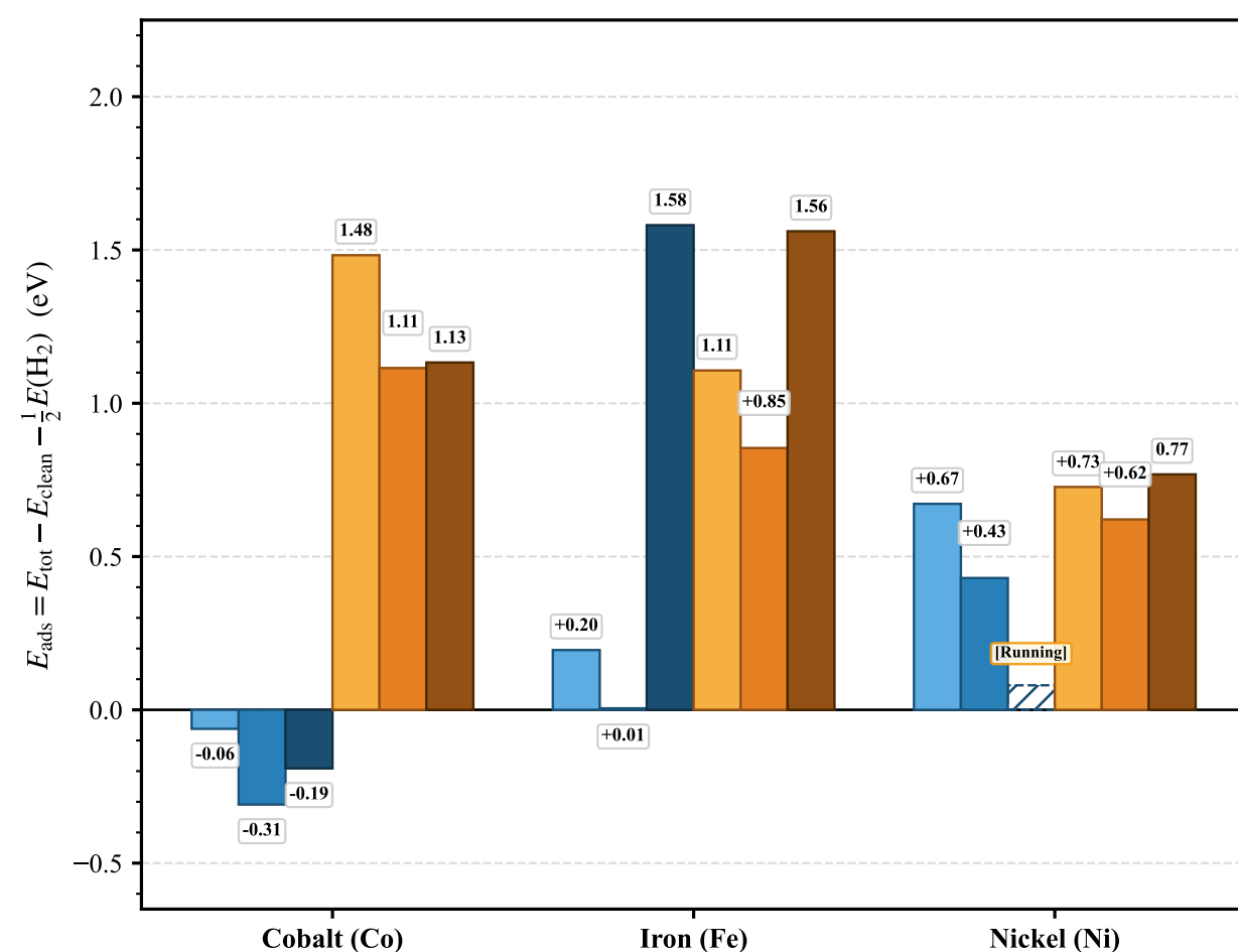
(b) Electronic Hydrogen Adsorption Energy ( E_{\text{ads}} )
