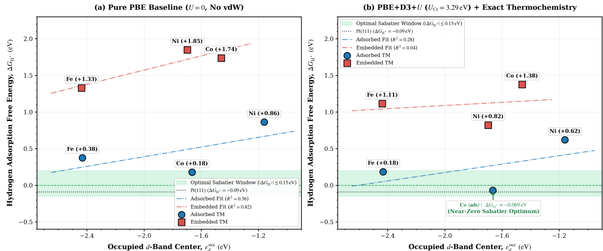
Figure 8: Occupied d -band center, \varepsilon_d^{\text{occ}} , versus hydrogen adsorption free energy, \Delta G_{\text{H}^*} , for surface-adsorbed and embedded Co, Fe, and Ni centers in monolayer \text{CrCl}_3 under (a) pure PBE baseline and (b) PBE+D3+ U ( U_{\text{Cr}} = 3.29 eV; with +U_{\text{all}} benchmark in Table 1) with explicit vibrational zero-point and entropic corrections. Linear fits are included only as visual guides because each coordination family contains three data points. Shaded green bands denote the optimal Sabatier catalytic window ( |\Delta G_{\text{H}^*}| \leq 0.15 eV) with the Pt(111) benchmark ( -0.09 eV) indicated by dotted horizontal lines.
