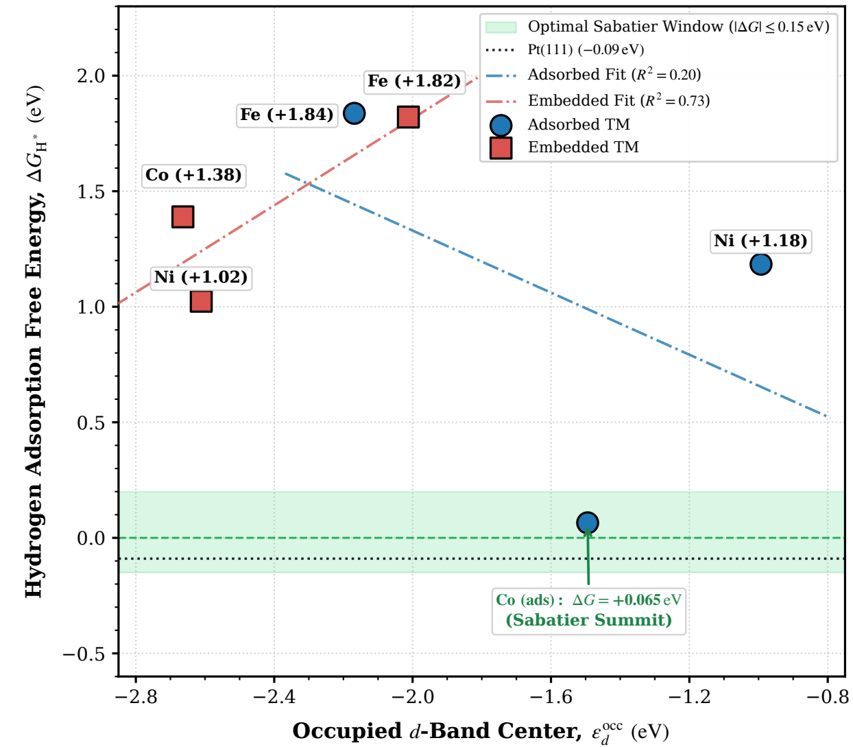
(c) Multi-Site +U_{\text{all}} ( U_{\text{Cr}}, U_{\text{TM}} = 3.29 eV)
