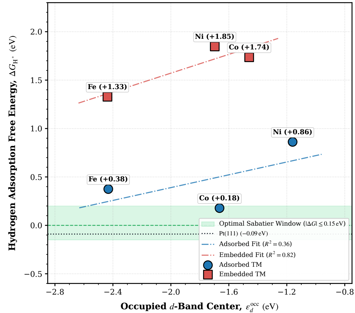
(a) Pure PBE Baseline ( U = 0 )
