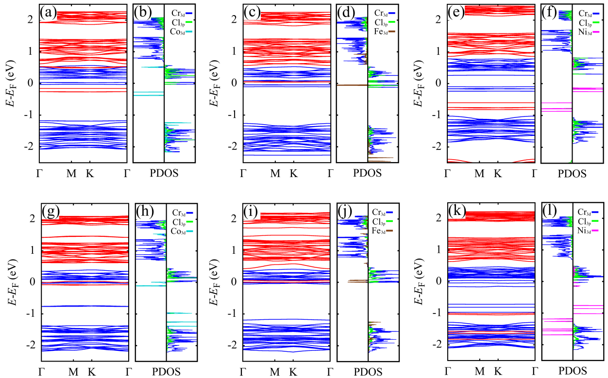
Figure 5: Spin-resolved band structures and projected densities of states of transition-metal-functionalized monolayer CrCl 3 . Panels (a,b), (c,d), and (e,f) correspond to surface-adsorbed Co, Fe, and Ni, respectively; panels (g,h), (i,j), and (k,l) correspond to the embedded configurations. Blue and red bands denote the spin-up and spin-down channels. The PDOS includes Cr-3 d , Cl-3 p , and TM-3 d contributions, and all energies are referenced to the corresponding Fermi level.
