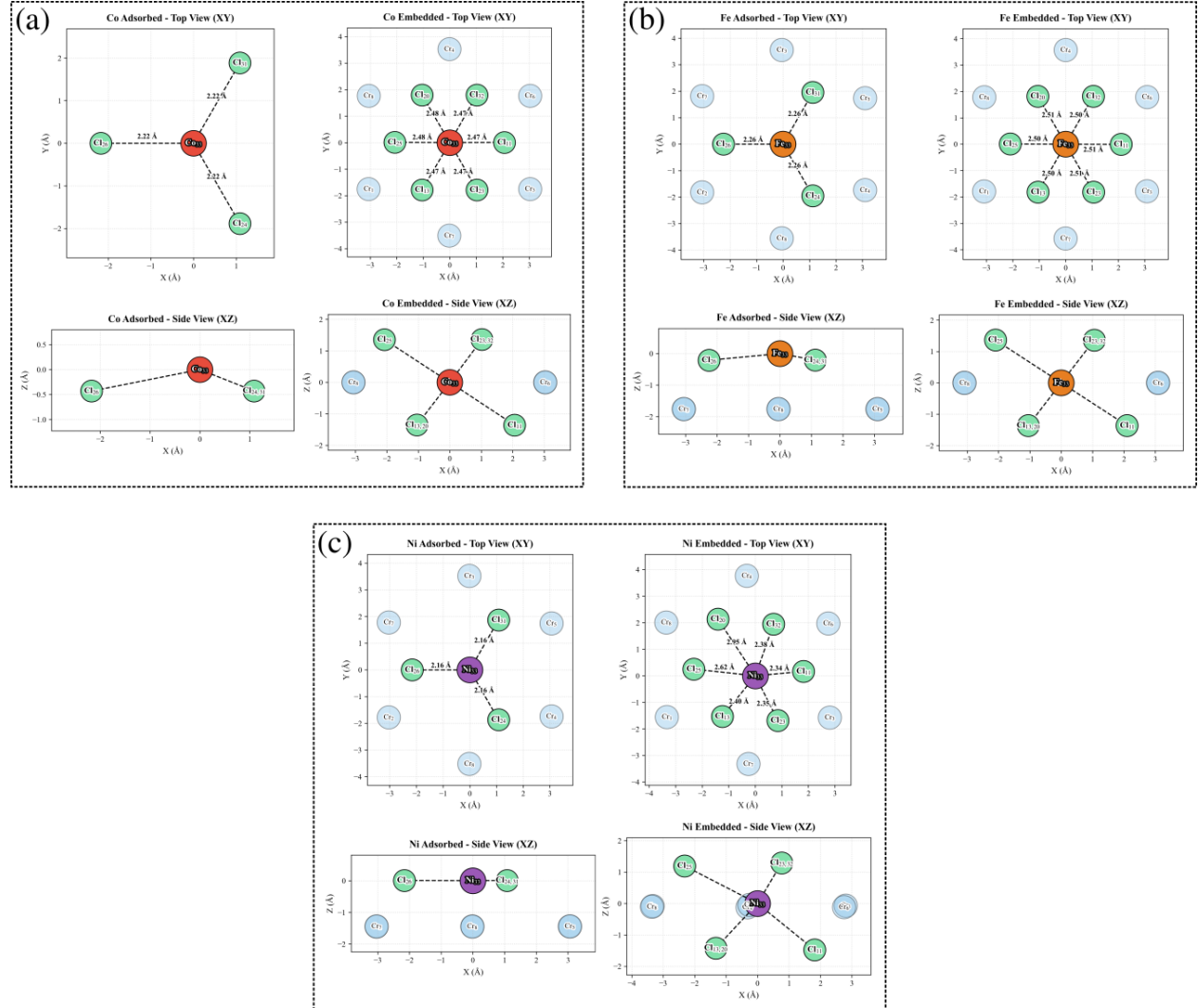
Fig. S1. Schematic top (XY) and side (XZ) views of the optimized local coordination geometries and TM-Cl bond lengths (Å) for (a) Co-, (b) Fe-, and (c) Ni-functionalized monolayer \text{CrCl}_3 in both adsorbed (hollow site, 3-fold coordinated) and embedded (6-fold octahedrally coordinated) configurations. Light blue, light green, and red/orange/purple spheres represent Cr, Cl, and transition-metal (Co, Fe, Ni) atoms, respectively.
