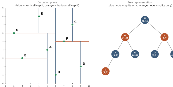
Figure 16: A 2D k-d tree: 8 points split by alternating axis (vertical first, horizontal next, and so on). Left: the resulting partition of the plane. Right: the same splits as a binary tree.
