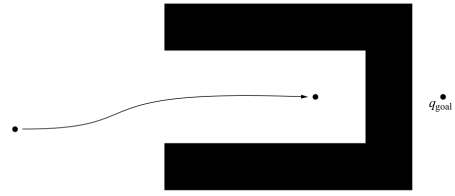
Figure 9: Failure case: inside a concave (horseshoe) obstacle, the repulsive gradient from the near wall exactly balances the attractive pull toward q_{goal} (cf. book Fig. 4.10).
