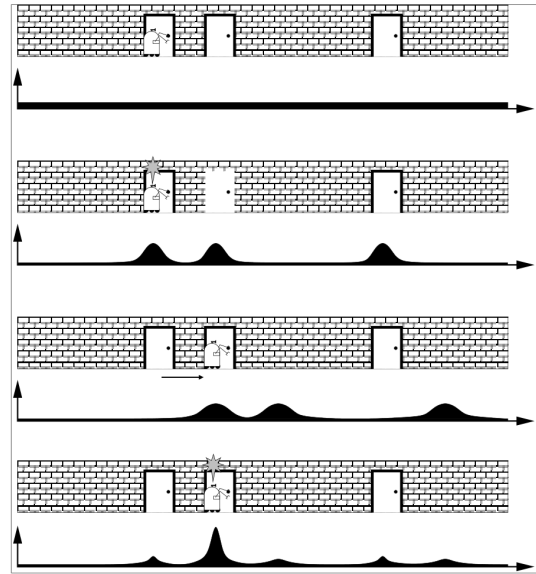
Figure 27: Global localization in a hallway with 3 doors: the belief starts uniform; sensing a door splits it into 3 equally-likely peaks; moving right predicts-forward and flattens each peak slightly; sensing a second door reinforces only the peak consistent with both sightings, leaving the robot confident of its true location — prediction spreads the belief out, update sharpens it (cf. book Fig. 9.1).
