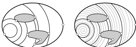
Figure 15: Curved-slice boustrophedon decomposition (cf. book Fig. 6.12).
