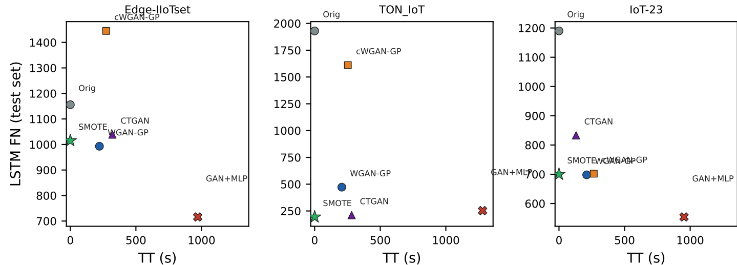
LSTM cost-effectiveness: FN on the test set vs. generator training time
