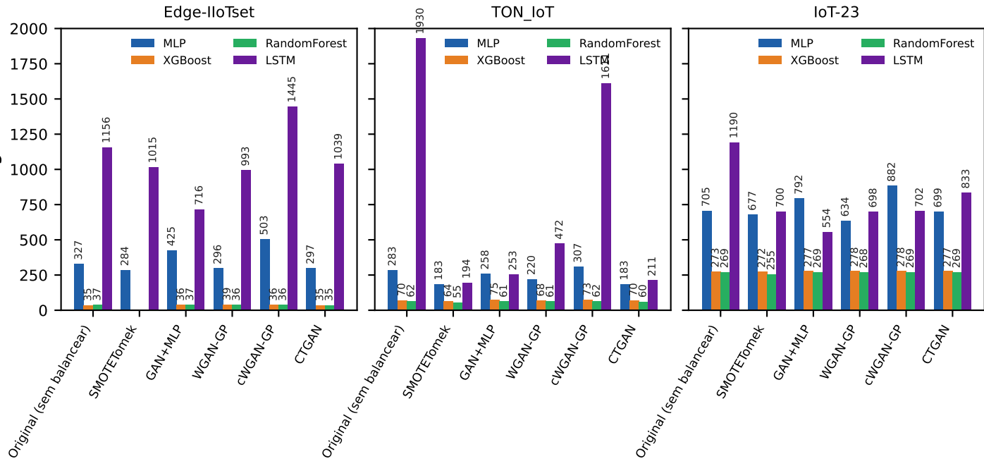
False negatives per model and balancing strategy (fixed test set)
