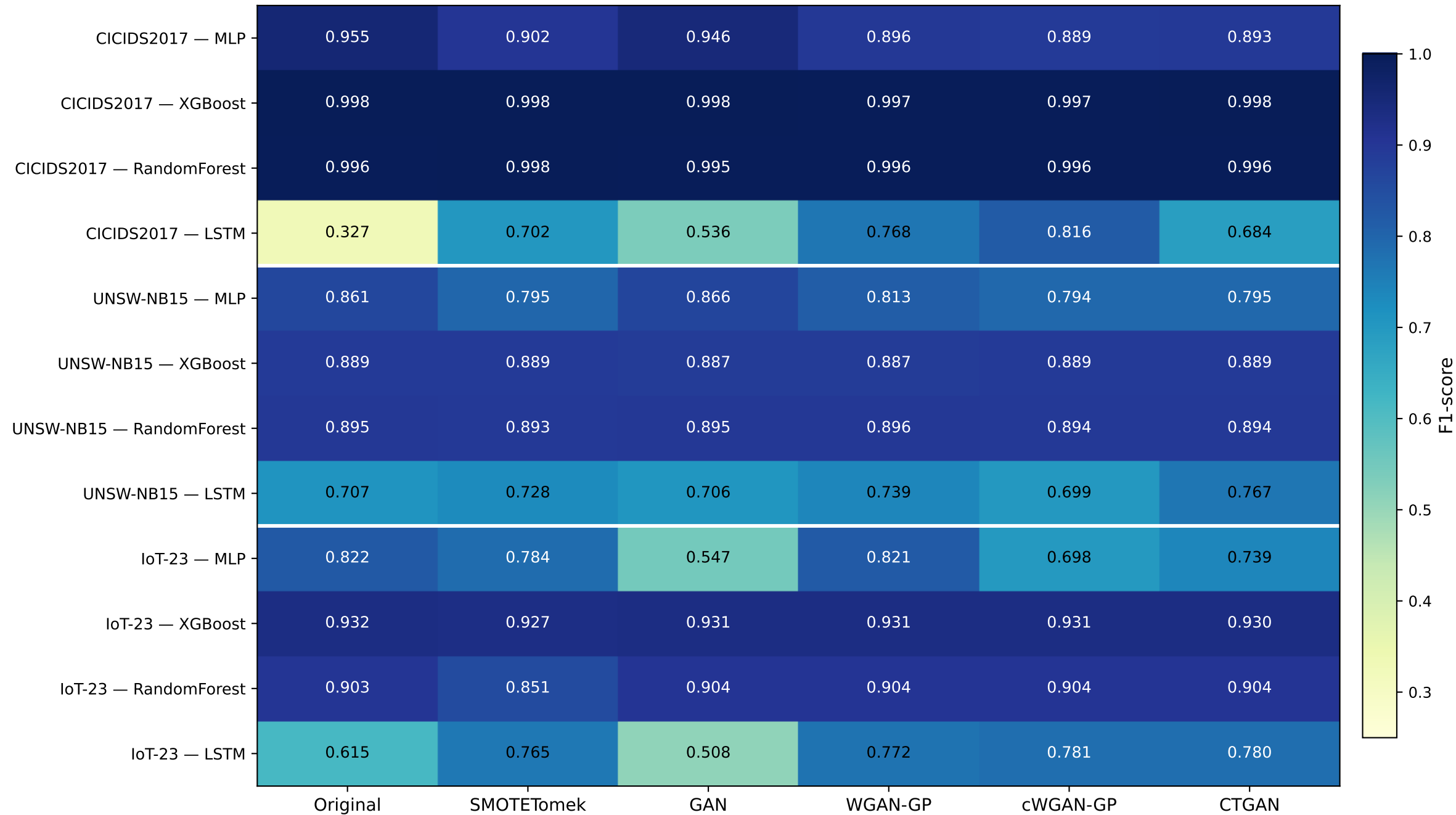
F1-score per dataset, model, and balancing strategy (test set, 12,000 flows)
