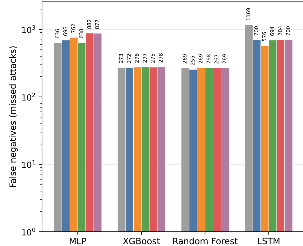
IoT-23
