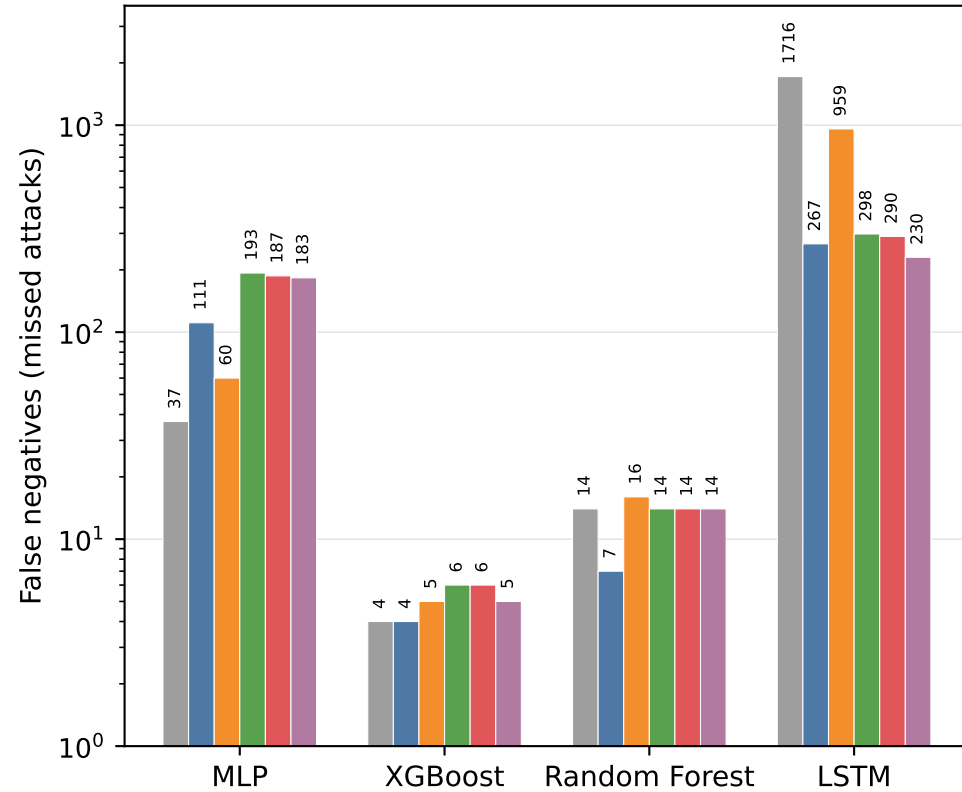
CICIDS2017
