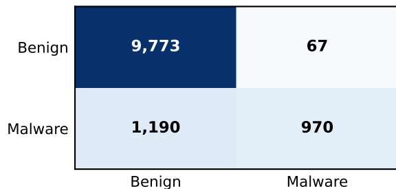
(e) IoT-23: Original
