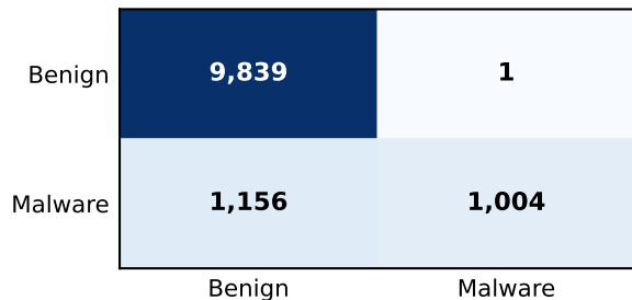
(a) Edge-IIoTset: Original
