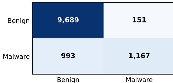
(b) Edge-IIoTset: Best balanced
