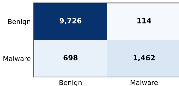
(f) IoT-23: Best balanced
