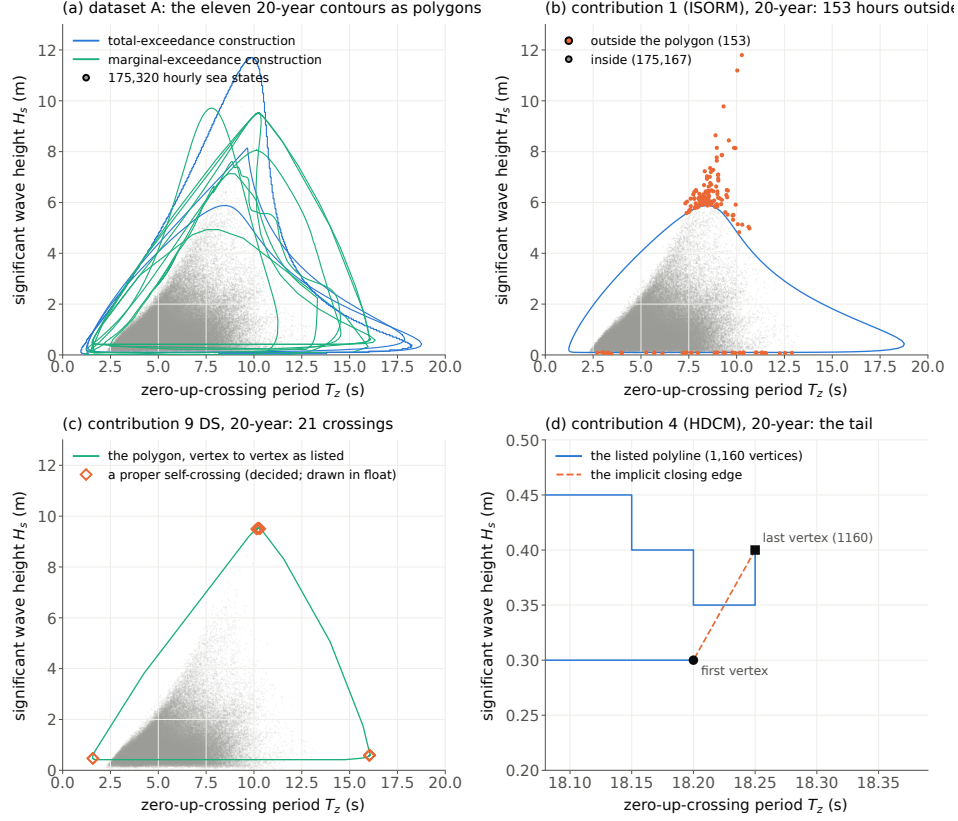
Figure 9: Dataset A of the contour benchmark. (a) The eleven 20-year contours as the polygons their files denote, each closed from its last vertex to its first, over the 175,320 hourly sea states. (b) Contribution 1’s ISORM contour with the 153 hours decided outside it marked; the drawing refuses to build if matplotlib’s own test on the same polygon does not reproduce the count. (c) Contribution 9’s direct-sampling contour drawn vertex to vertex in file order, with its 21 proper self-crossings (the count is decided; the positions are drawn in floating point). (d) The tail of contribution 4’s highest-density contour: the listed polyline ends at the square, and the implicit closing edge back to the circle, the longest edge of the polygon, crosses the staircase.
