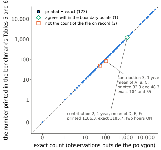
Figure 8: The 176 numbers printed in the contour benchmark’s two tables against the exact counts (both axes symmetric-logarithmic). 173 lie on the diagonal; the one that agrees within the two boundary points and the two that are not the count of the file on record are marked.
