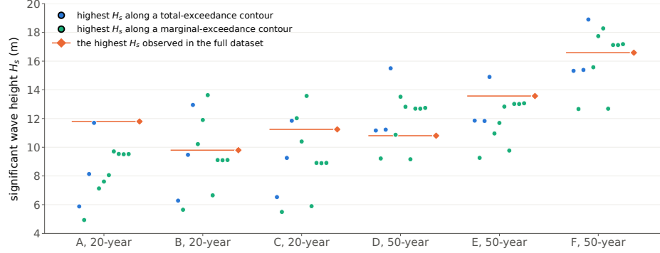
Figure 3: For each dataset, the highest significant wave height along each of the eleven long-return-period contours (a literal read from the file: a linear function on a polygon peaks at a vertex) against the highest wave height observed in the full dataset.
