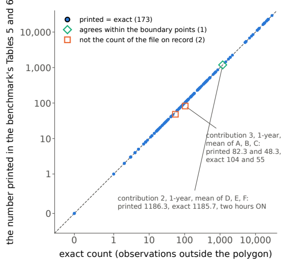
Figure 1: The 176 numbers printed in the benchmark’s Tables 5 and 6 against the exact counts (both axes symmetric-logarithmic). 173 lie on the diagonal; the one that agrees within the two boundary points and the two that are not the count of the file on record are marked.
