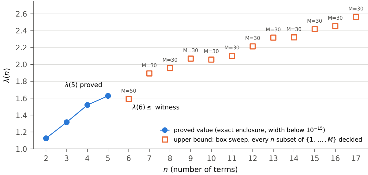
Figure 1: The certified \lambda landscape, n = 2, \dots, 17 . Filled marks are proved values (Mercer at n = 2, 3 ; [11] at n = 4 ; this paper at n = 5 ). Hollow marks are the upper bounds of Table 4, each the best set in an exhaustive sweep of every n -subset of \{1, \dots, M\} ; the sequence may lie below any of them. The value at n = 6 is the witness bound of Theorem 3.
