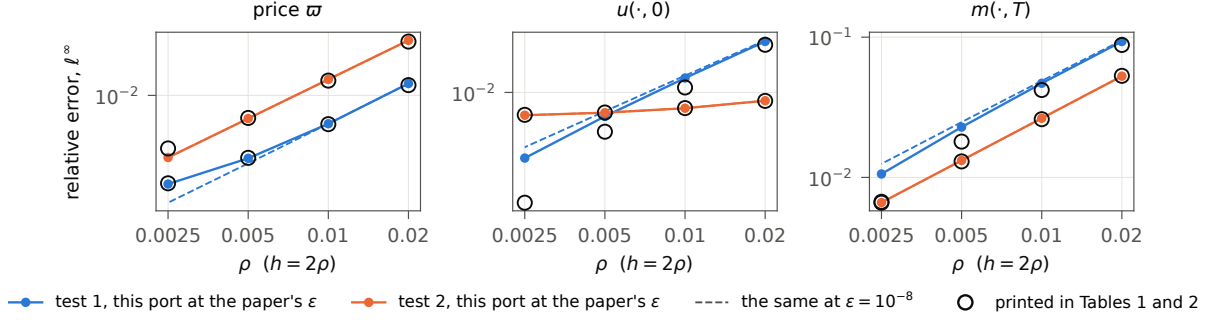
Figure 1: The relative errors of Table 1 against the mesh, logarithmic axes. Filled marks: this port at the paper's tolerance; dashed: the same at \varepsilon = 1 \times 10^{-8} ; hollow: printed. The printed price of test 1 sits on the port's line at every mesh. The port's price errors halve as \rho halves — ratios 2.04, 2.02, 2.01 (test 1) and 2.00, 2.00, 2.00 (test 2) at the tight tolerance — where the printed test-1 ratios are 2.00, 1.82, 1.57.
