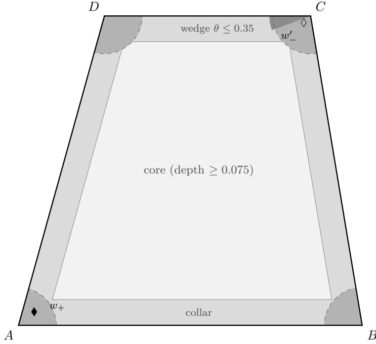
Figure 1: The zone map. Core: value argument against the witness w_+ (max side) and w'_- (min side), margins 5.4 \cdot 10^{-2} and 1.2 \cdot 10^{-2} . Collar: 2,166 cells, reflected bounds, zero residual. Tips (radius 0.11, dashed): exact corner expansions — A dies radially, B and D by value, C by a no-critical-point sector plus the wedge, where \hat{\varphi}_{nn} \geq 13.04 .
