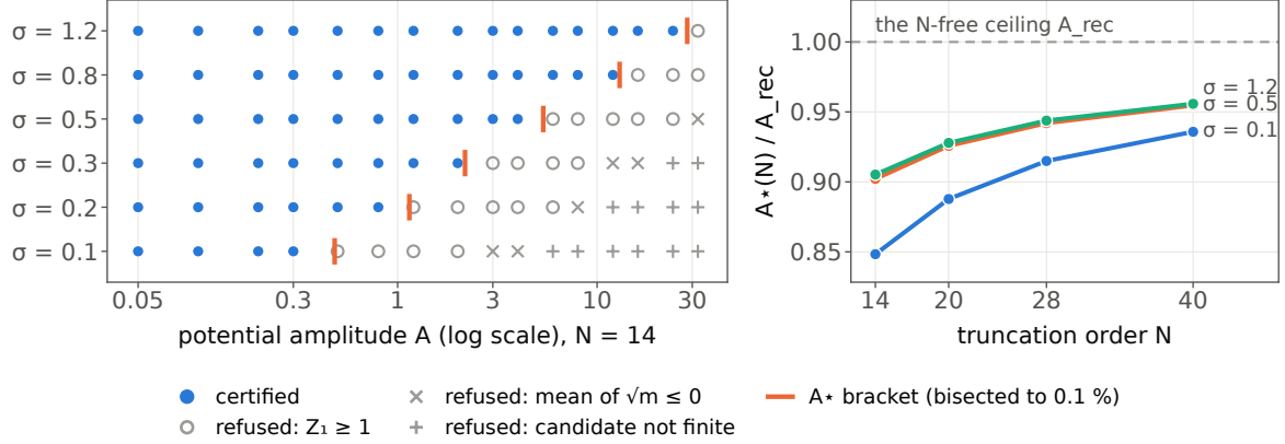
Figure 3: Left: the six amplitude ladders at N = 14 on a logarithmic axis, 16 amplitudes from 0.05 to 32 evaluated at every viscosity; every ladder is certified up to a boundary and refused beyond it, the first refusal always Z_1 \geq 1 , the boundary bisected to a tenth of a percent (orange). Right: the certified boundary relative to the N -free ceiling A_{\text{rec}} rises with the truncation order at every viscosity and stays below one; the lines join decided brackets and are a trend, not a law.
