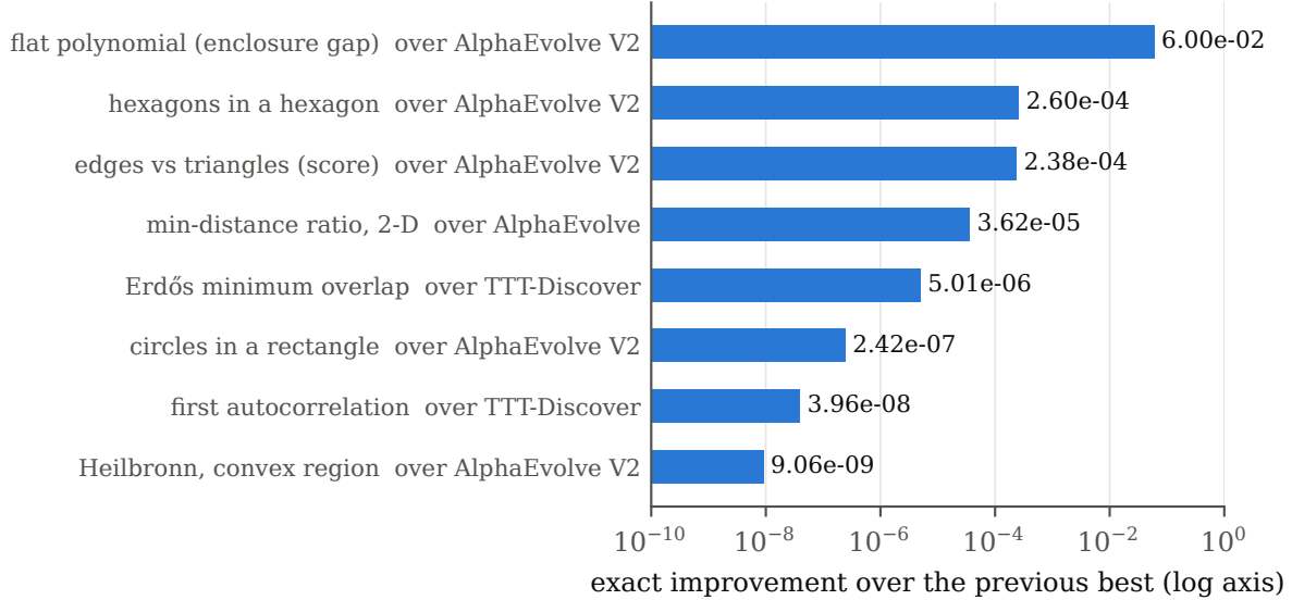
Figure 2: The 8 improvements over the previous best, each an exact difference of two rationals (for the flat polynomial, the gap between two disjoint certified enclosures), on a log axis. All are positive; the smallest, 9.06 \times 10^{-9} on the Heilbronn configuration, is nine digits in and real. The largest exact difference, 2.6 \times 10^{-4} , is the hexagon side; the benchmark score (edges vs triangles) is 2.38 \times 10^{-4} .
