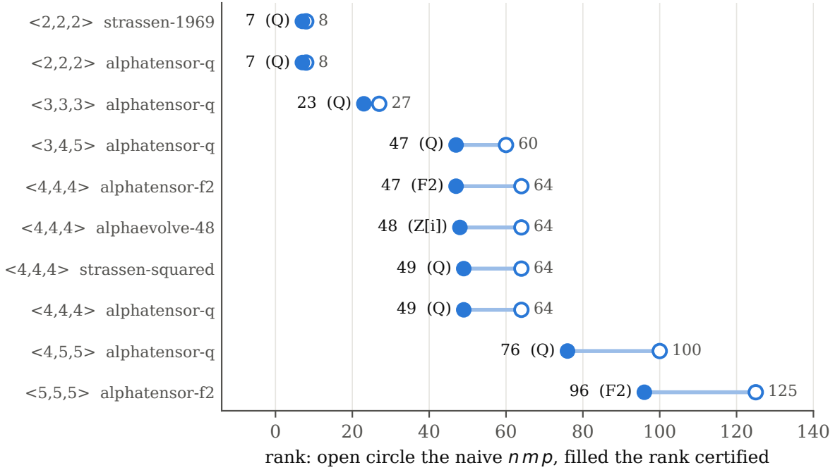
Figure 1: The ten verified rows, each drawn from the naive rank of its shape to the rank certified, with the ring beside it. The ring is not decoration: the two \mathbb{F}_2 rows are refuted over \mathbb{Q} .
