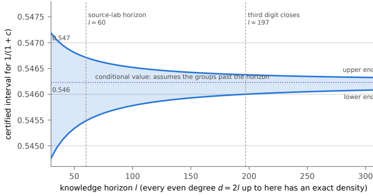
Figure 1: The certified interval for 1/(1+c) against the knowledge horizon l , every point re-assembled in exact rationals by the bracket module and rounded outward to twelve decimals: the band is the interval, the hairlines the decimal cells, the dotted line the conditional value of Section 7, which assumes the groups past the horizon and is drawn in a different style for that reason. The third decimal closes at l = 197 . Data: paper/tex/fig/erdos290-squeeze.json .
