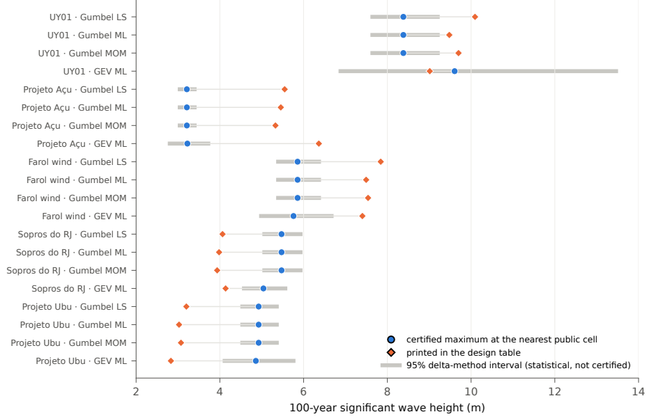
Figure 7: Twenty printed 100-year waves of a design table (Bhaskaran et al., 2023) against the certified fit at the nearest public cell, with the latter’s 95% delta-method interval. The difference measures the distance between two hindcasts at two points; the certificate makes it a number per row.
