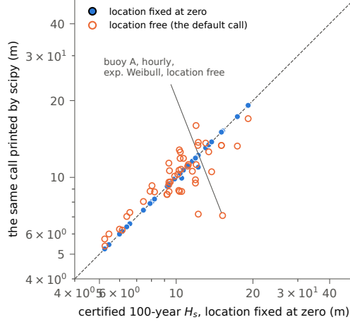
Figure 6: The 100-year level printed by the library against the certified maximum on the same block maxima, for the four families with a scale parameter on the three buoys at five blocks: location fixed at zero (filled) and the default call with a free location (hollow). The dashed line is equality.
