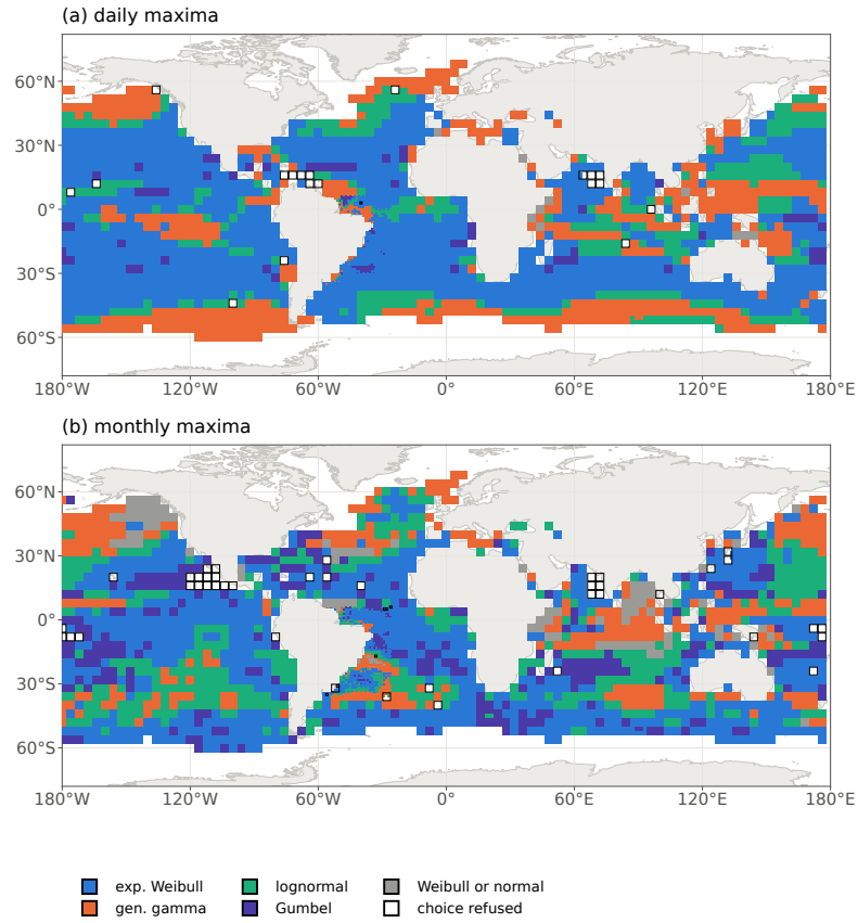
Figure 2: The family the Anderson–Darling statistic selects among the six at every open-sea cell, (a) daily and (b) monthly maxima; a hollow square is a refused choice. Cells are drawn as squares centred on their node: 4^\circ on the global lattice, 1^\circ on the Brazilian margin. The Weibull and the normal, selected at few cells, share one colour.
