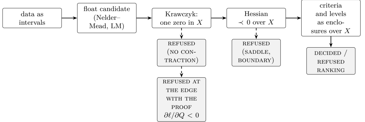
Figure 1: The certificate of one fit. A float search only proposes; the Krawczyk operator and the second-order test decide; every statistic is an interval extension over the certified box X . A refusal is a recorded result with its reason, and the generalized gamma can be refused at its lognormal limit only with the boundary proof of Section 3.4.
