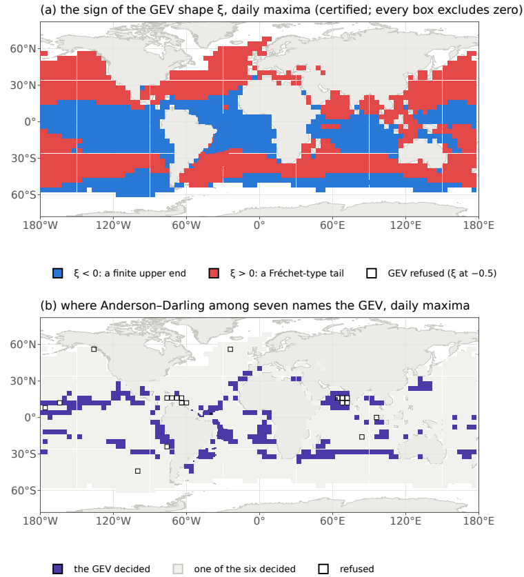
Figure 5: The seventh family on the daily maxima. (a) The sign of the GEV shape \xi , certified: below zero (a finite upper end) or above zero (a Fréchet-type tail); no certified box contains zero. (b) The cells where the Anderson–Darling statistic, applied to the seven families by the rule of Section 3.3, names the GEV.
